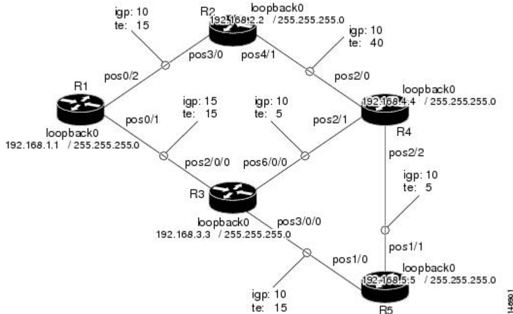
Figure 4 Network Topology
