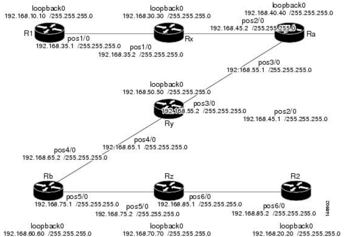
Figure 6 Router Topology
