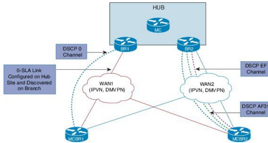
Figure 8: Probing on Zero SLA
