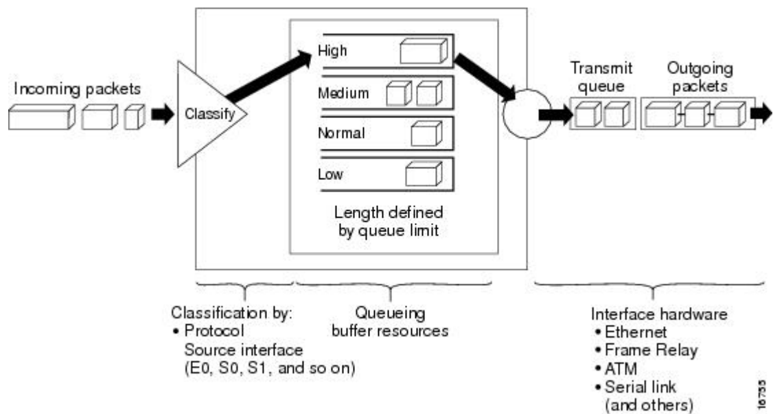
Figure 3: Priority Queueing
