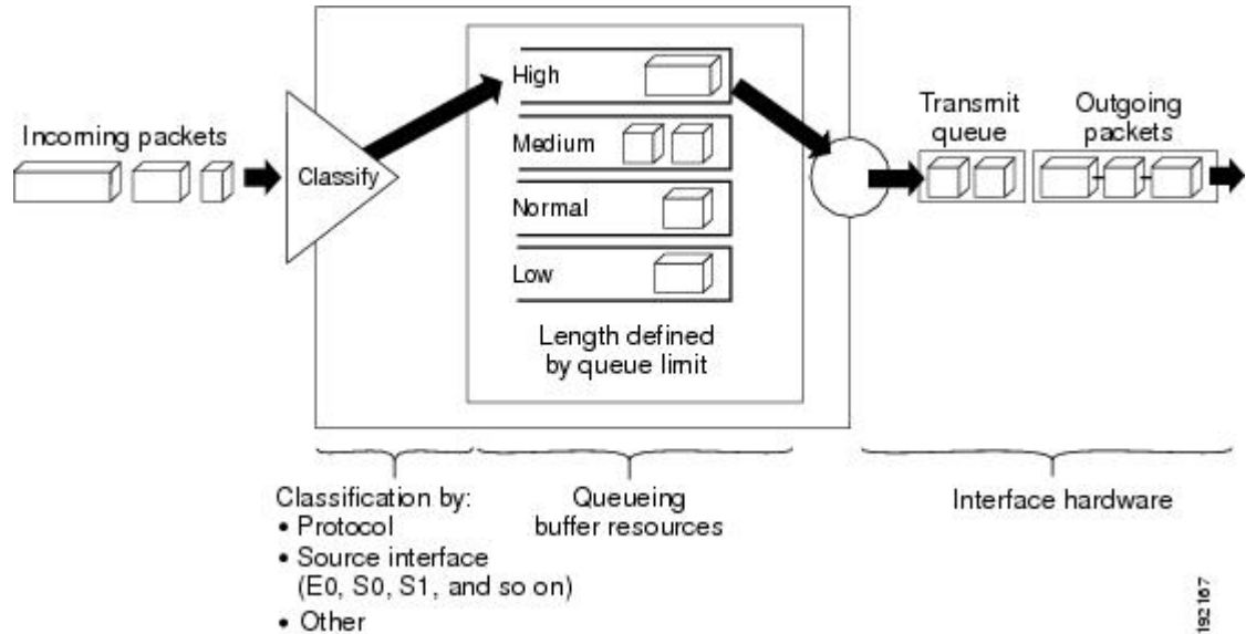
Figure 2: Priority Queuing
