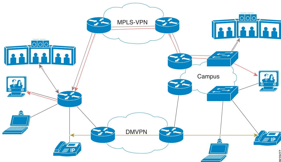
Figure 32 Application-Aware Path Selection
