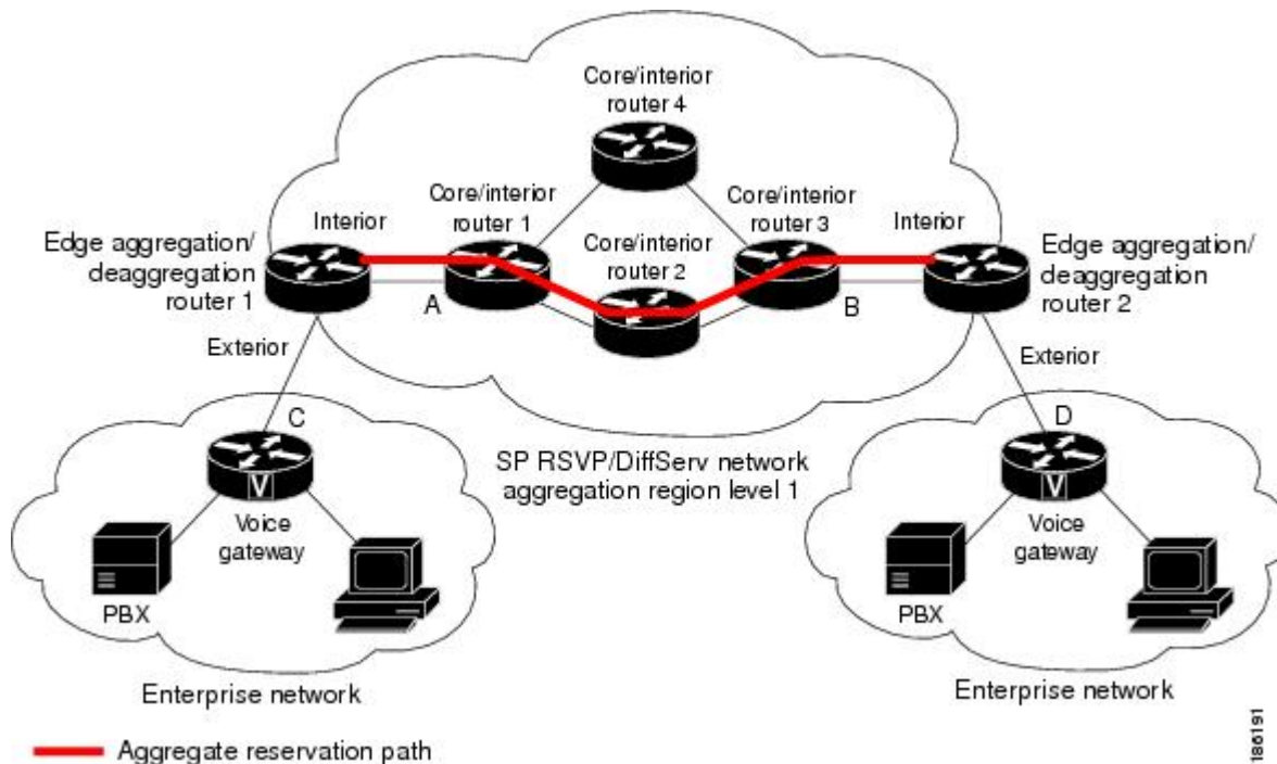
Figure 28 RSVP Aggregation Network Overview
