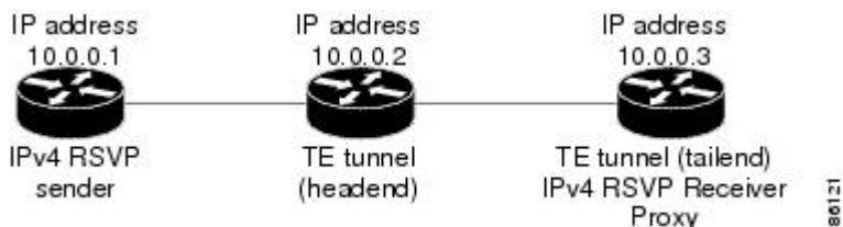
Figure 31 Sample TBAC Network
