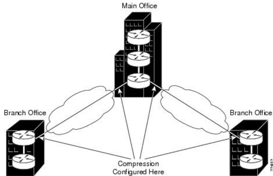
Figure 18 Configuring Compression
