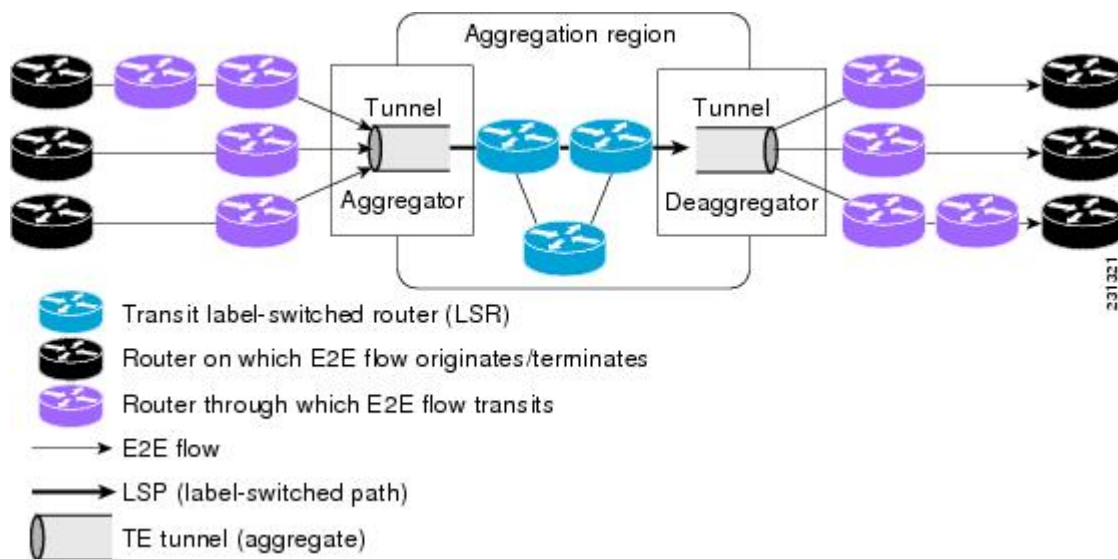
Figure 30 TBAC Overview
