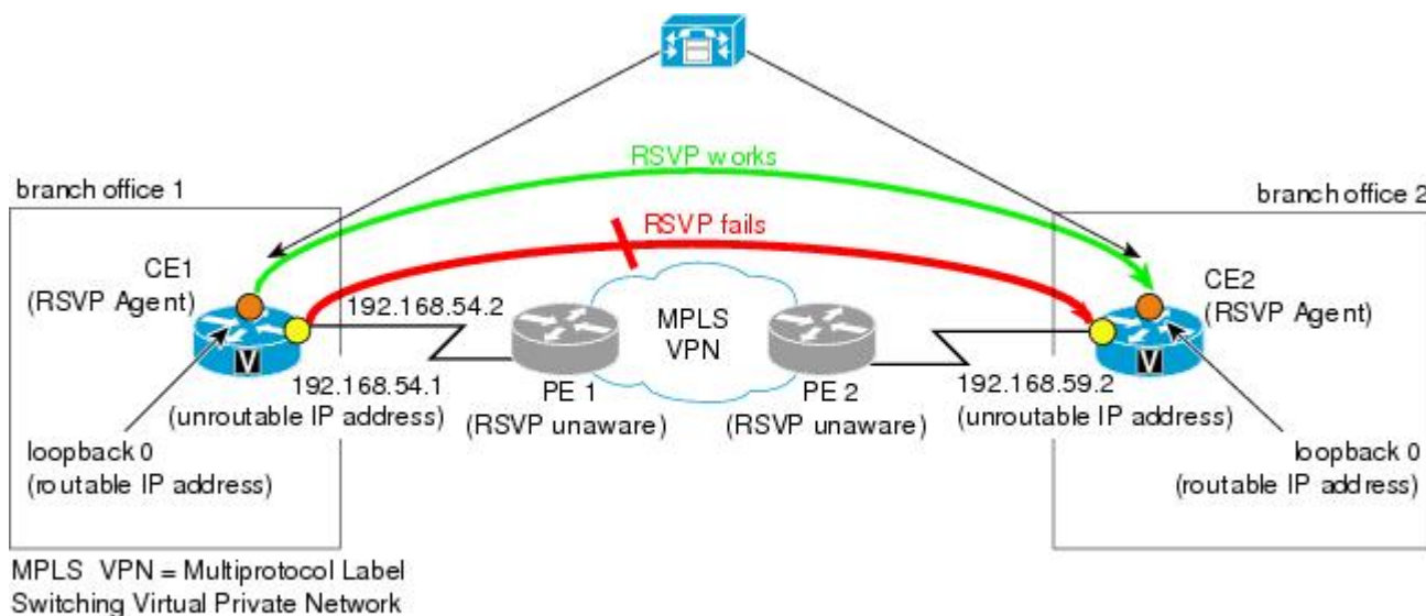
Figure 17 Sample PHOP Network with Unified Communications Manager (CM)
