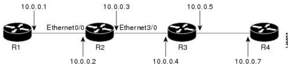
Figure 19 Sample Network with Application Identities and Local Policies
