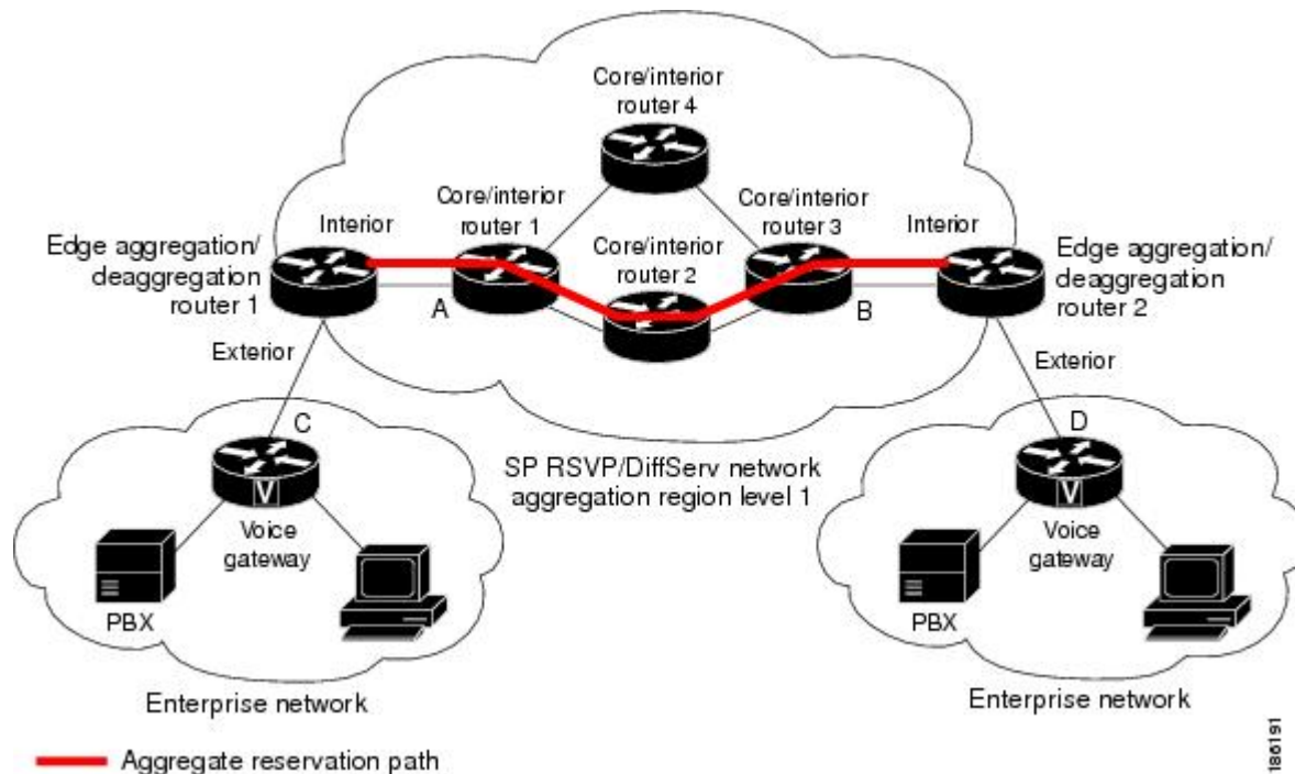
Figure 22 RSVP Aggregation Network Overview
