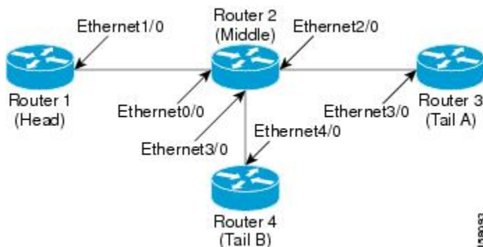
Figure 21 Sample Network with an Interface-Based Receiver Proxy Configure
