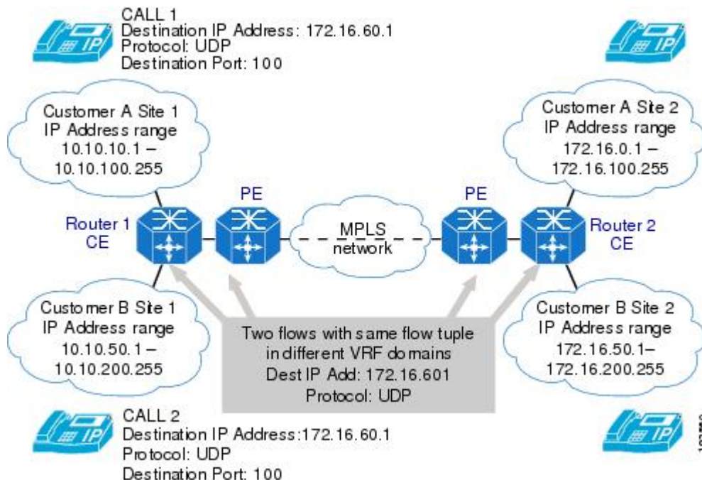
Figure 26 RSVP VRF Deployment in VRF-Lite Network
