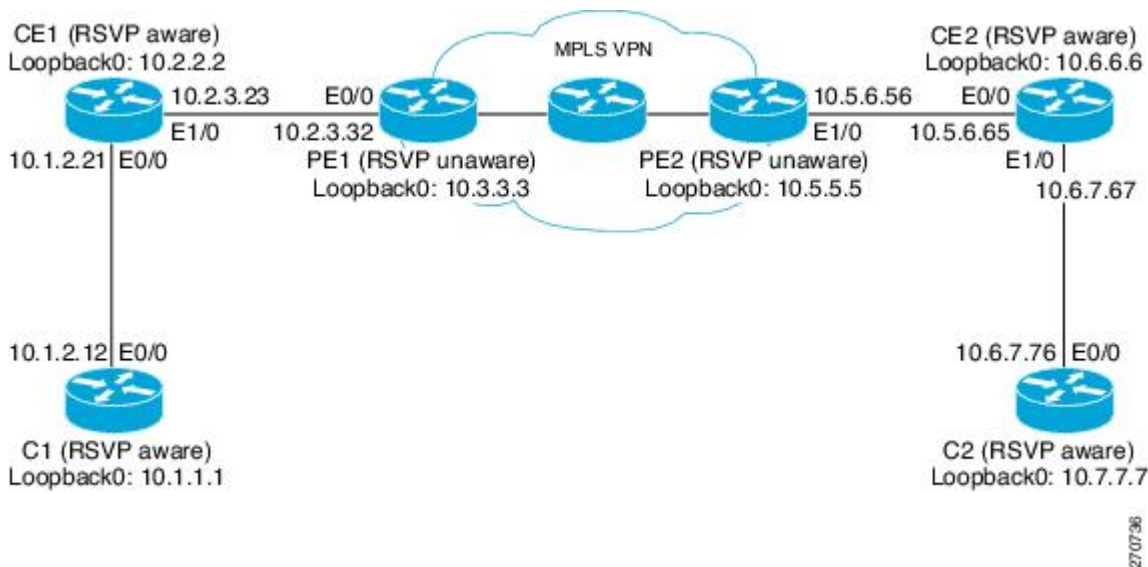
Figure 18 Sample PHOP Network
