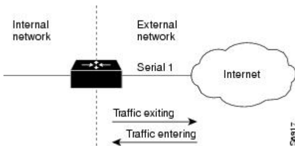
Figure 3 Simple Topology--CBAC Configured at the External Interface
