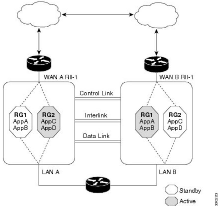
Figure 1: Asymmetric Routing Scenario
