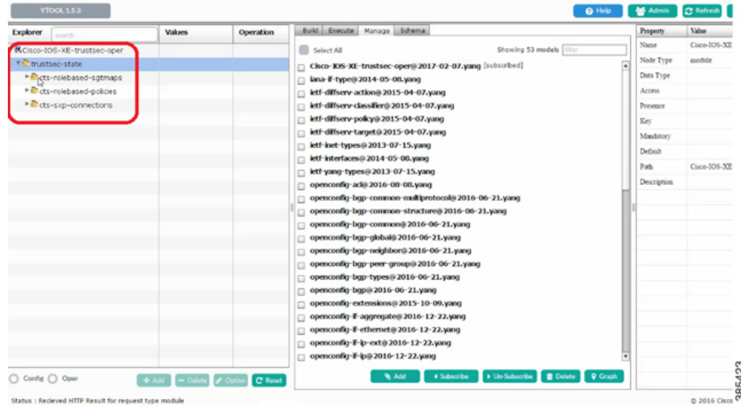
Figure 4: Subscribe Schema
