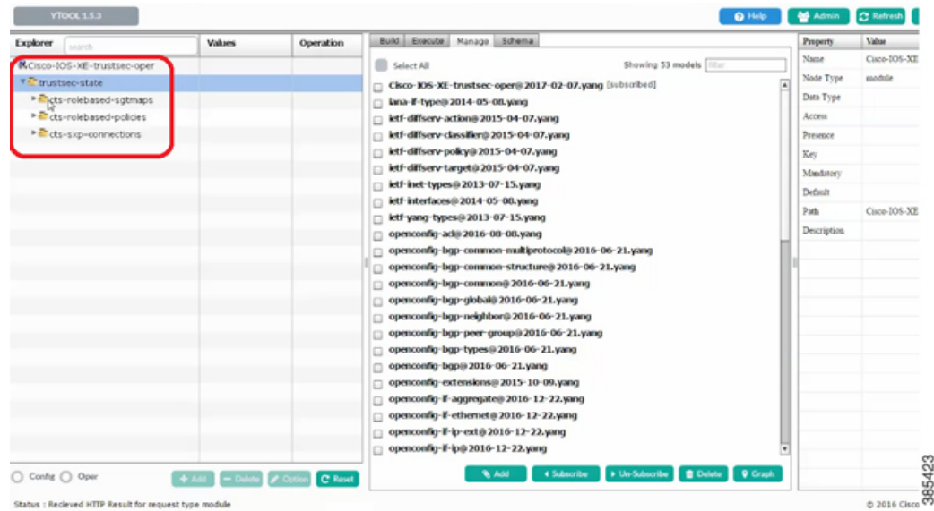
Figure 11: Subscribe Schema
