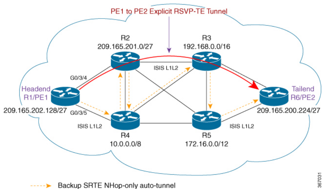
Figure 28: Explicit RSVP-TE Tunnel
