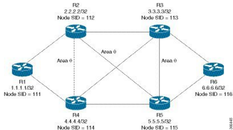
Figure 1: Intra Area Tunnel
