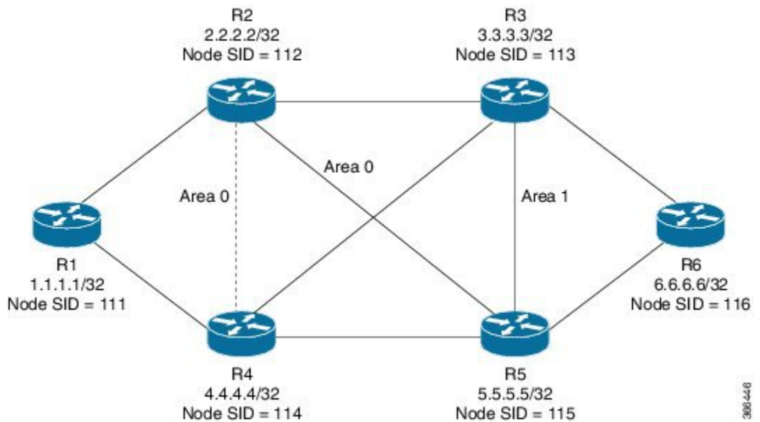
Figure 2: Inter Area Tunnel
