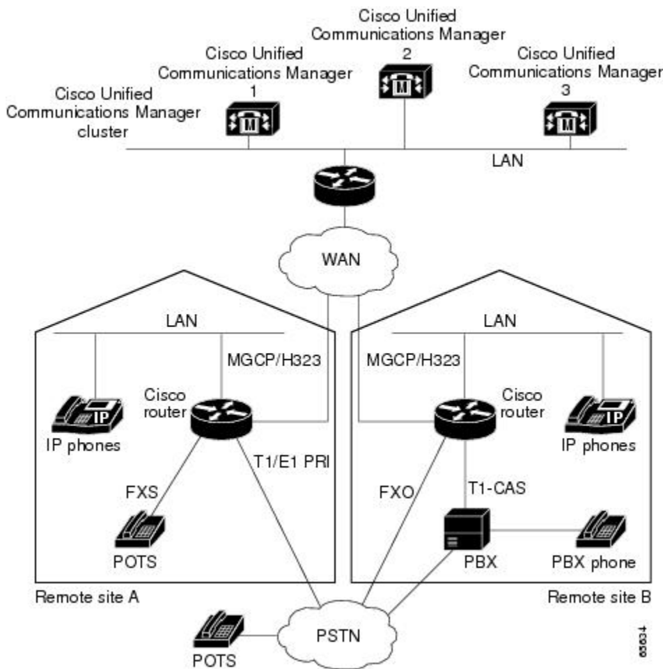
Figure 2: Typical VoIP Network Topology Supporting the MGCP Gateway Fallback Feature
