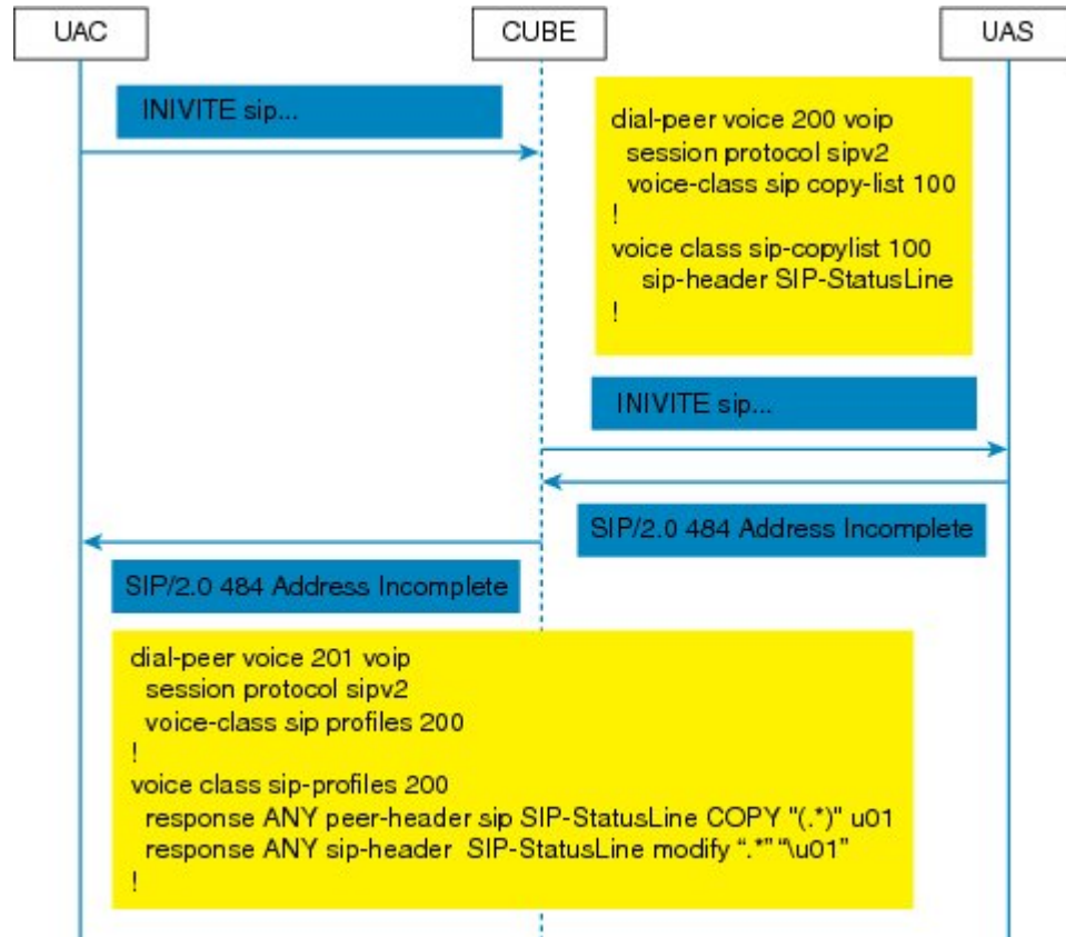
Figure 14: Call Flow for Copying the Status Line from the Incoming SIP Response to the Outgoing SIP Response
