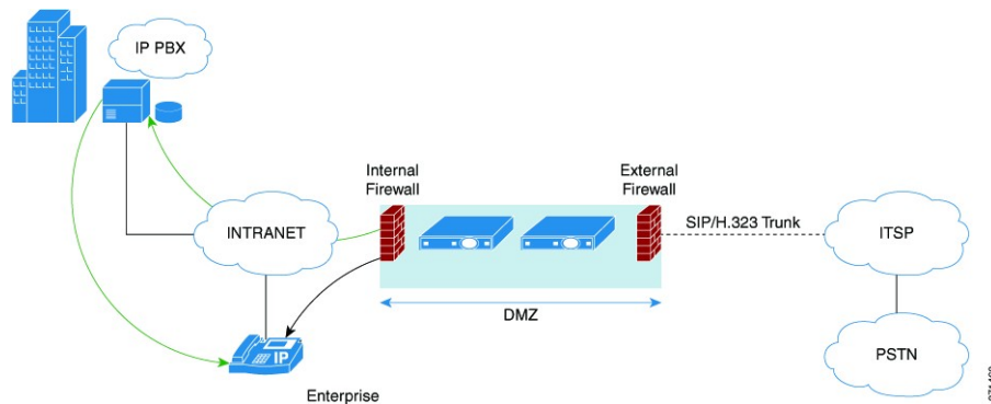
Figure 3: SIP/H.323 Trunking
