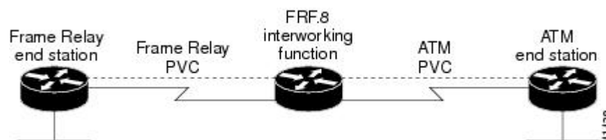
Figure 21 Frame Relay-to-ATM Service Interworking (FRF.8)
