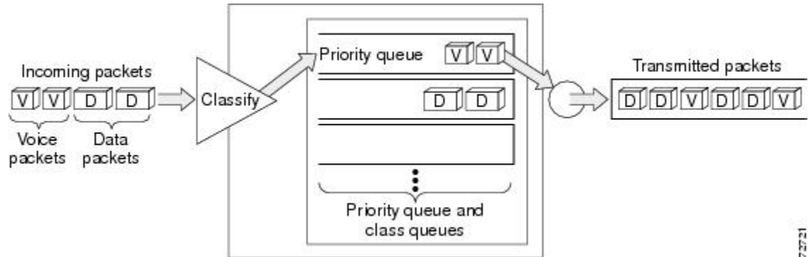
Figure 15 Frame Relay Queueing and Fragmentation at the Interface
