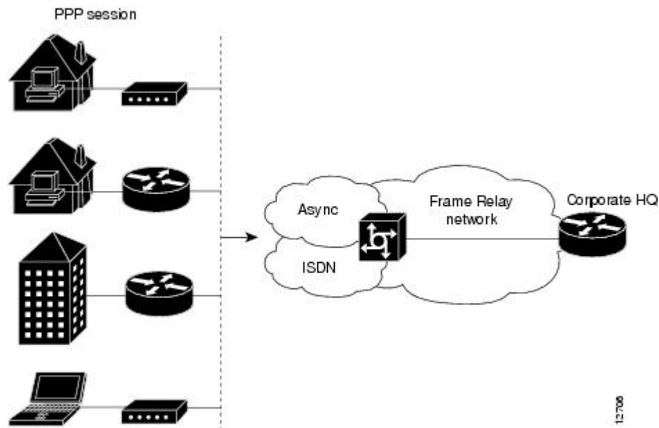
Figure 17 PPP over Frame Relay Scenario
