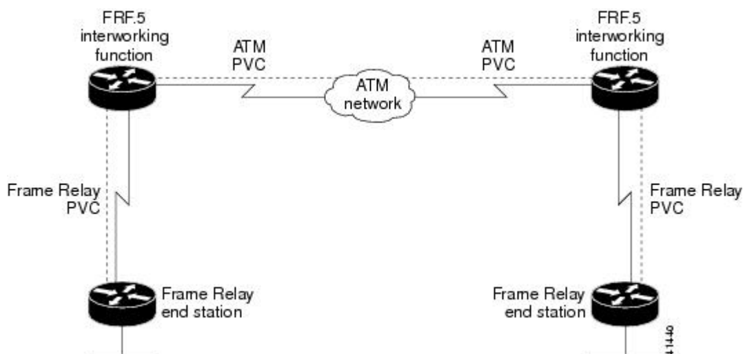
Figure 20 Frame Relay-to-ATM Network Interworking (FRF.5)
