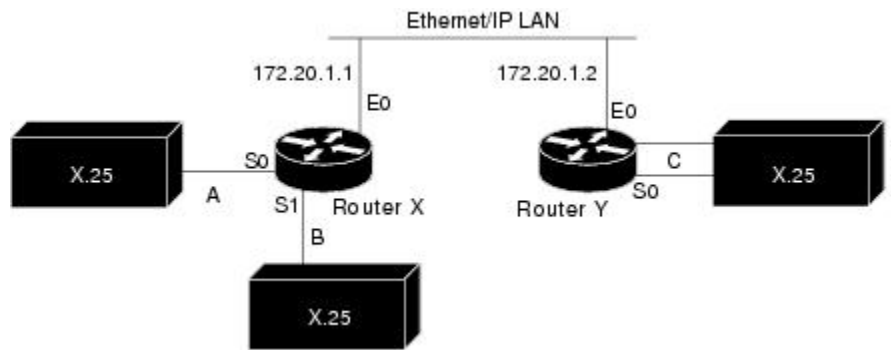
Figure 14: PVC Switching over XOT
