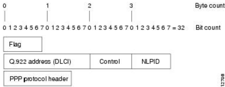
Figure 19: PPP over Frame Relay Frame Format
