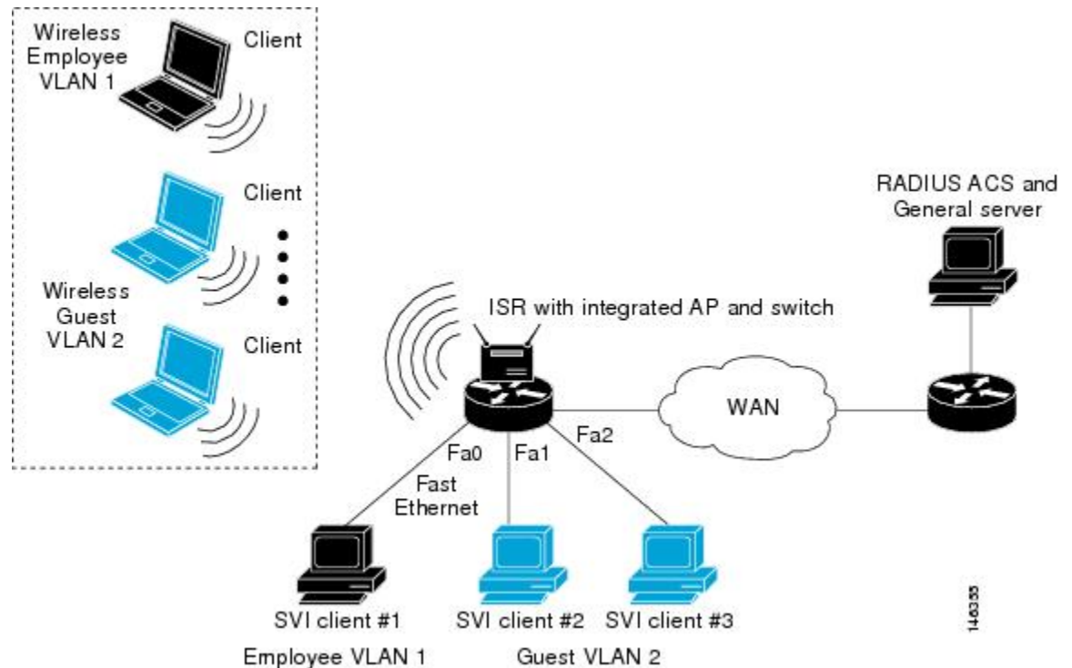
Figure 1: LAN and VLAN Segmentation with Wireless Devices
