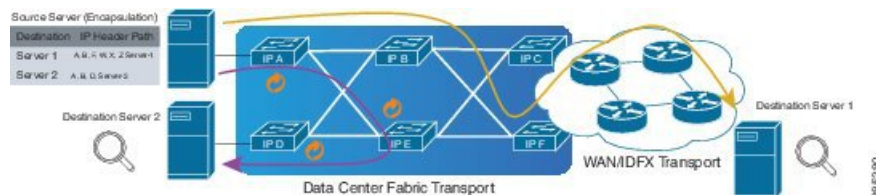
Figure 12: IP-in-IP Decapsulation Through a Data Center Network
