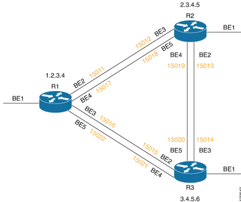
Figure 22: VPWS over SR-TE
