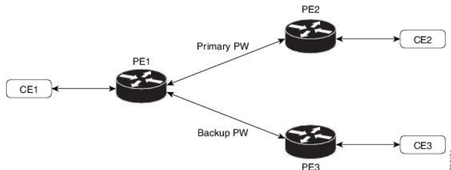
Figure 14: Pseudowire Redundancy
