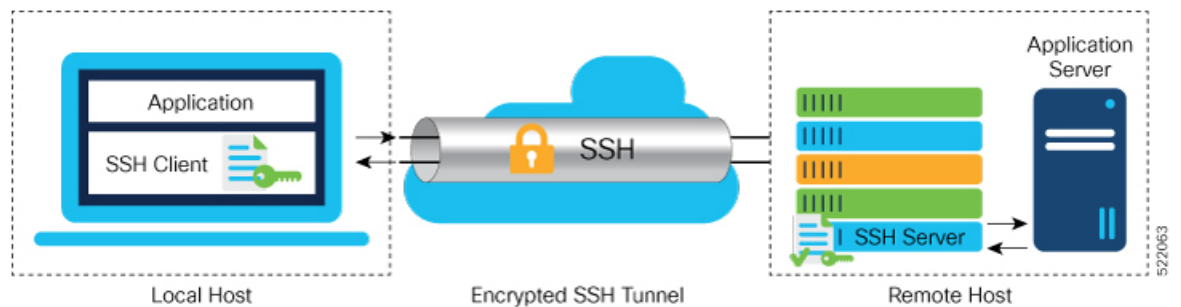
Figure 17: SSH Port Forwarding
