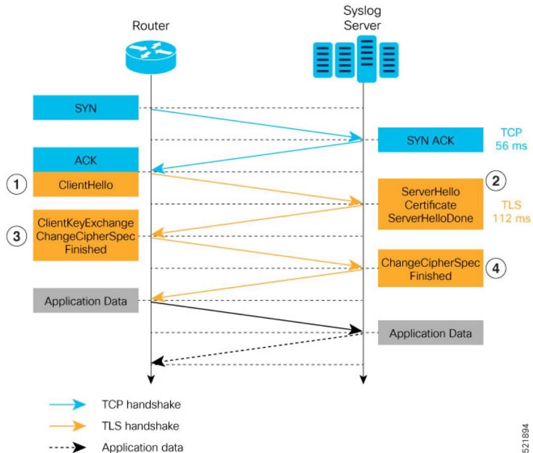
Figure 7: TLS Handshake
