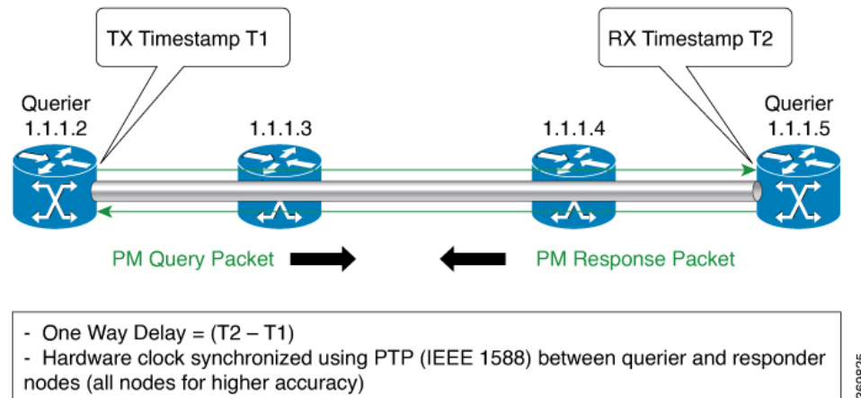
Figure 50: Performance Measurement for SR Policy End-to-End Delay
