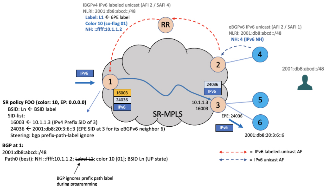
Figure 32: EPE Traffic-Engineered Path
