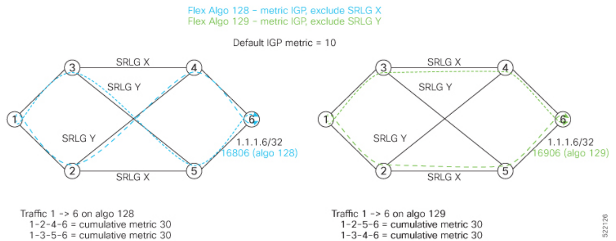
Figure 43: Flex Algo with Exclude SRLG Constraint
