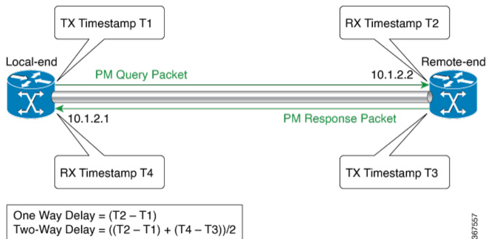
Figure 48: Performance Measurement for Link Delay
