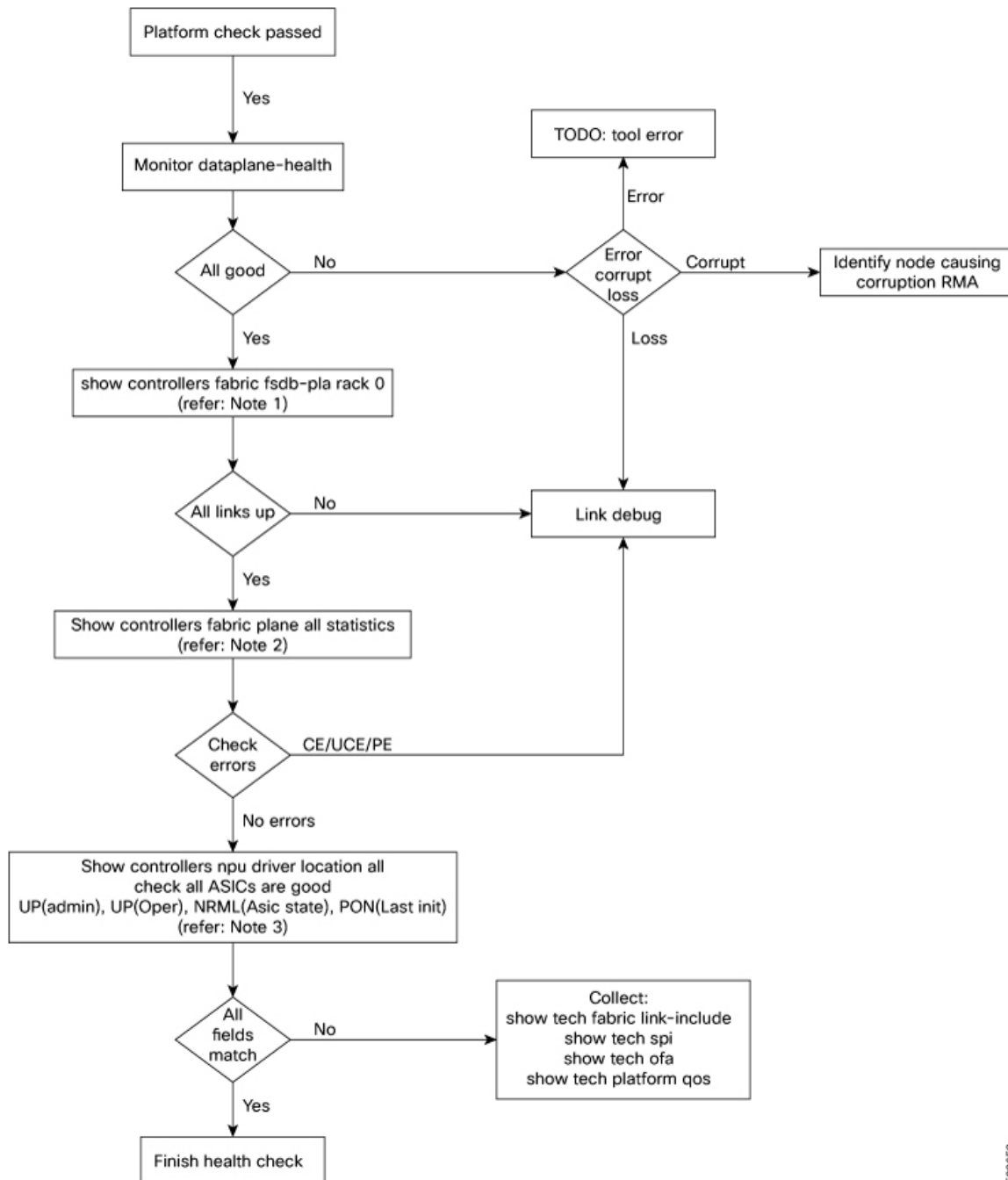
Figure 10: Troubleshooting Flowchart
