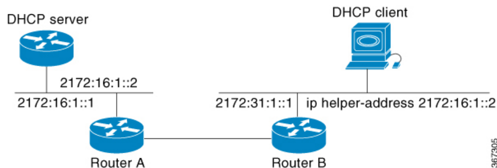
Figure 11: Forwarding UDP Broadcasts to a DHCPv6 Server Using a Helper Address
