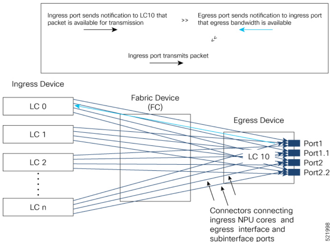
Figure 3: The Ingress Traffic Management Model
