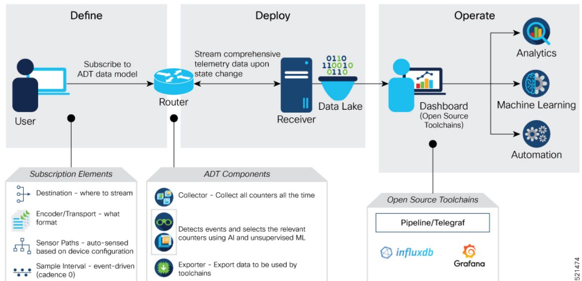
Figure 12: AI-Driven Telemetry
