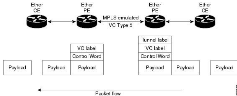
Figure 11: Ethernet Port Mode Packet Flow
