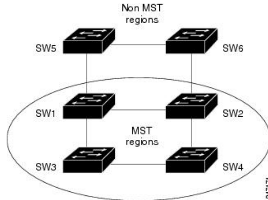
Figure 33: MST Interaction with Non-MST Regions
