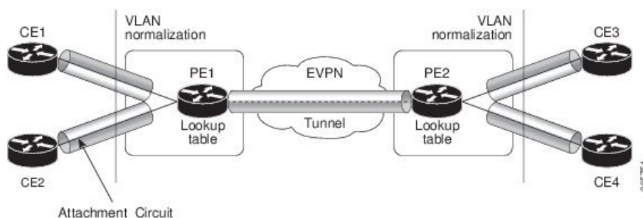
Figure 17: Flexible Cross-Connect Service
