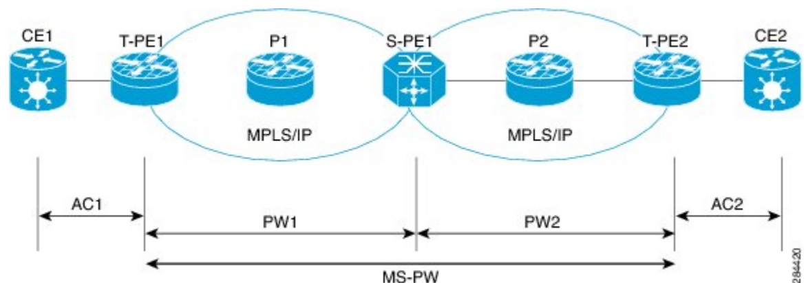
Figure 21: Multisegment Pseudowire
