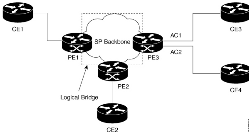
Figure 23: Split Horizon Group 2
