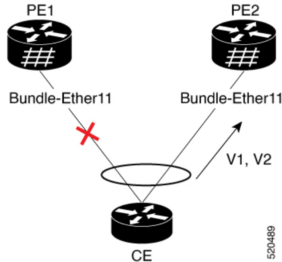
Figure 36: EVPN Port-Active Multihoming
