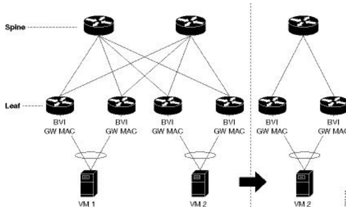
Figure 53: EVPN IRB
