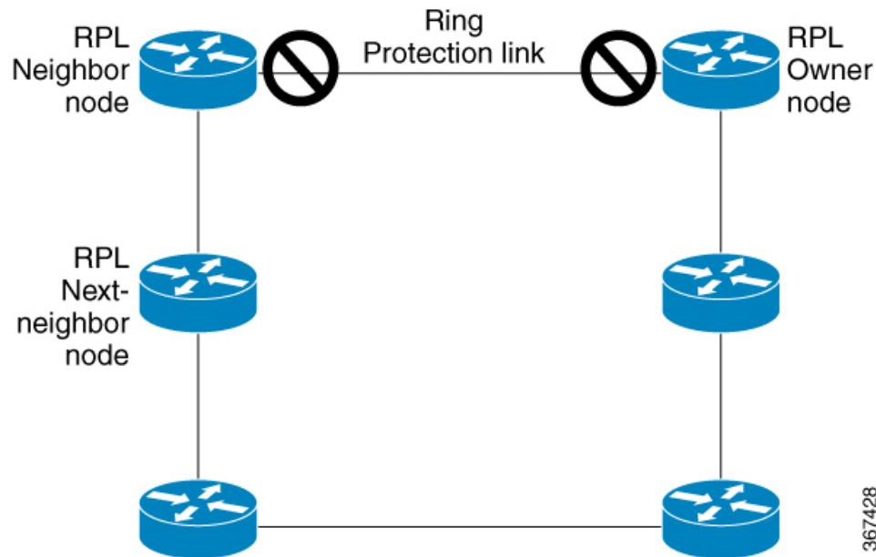
Figure 24: G.8032 Ethernet Ring
