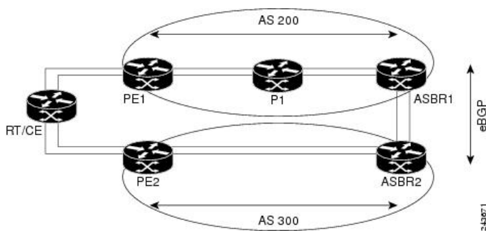
Figure 13: EoMPLS over Inter-AS: Basic Double AS Topology
