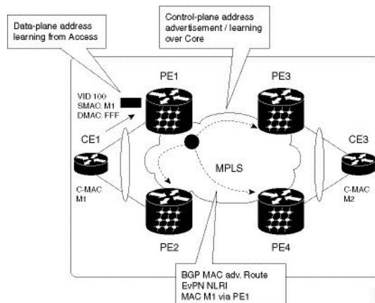
Figure 35: EVPN Operation
