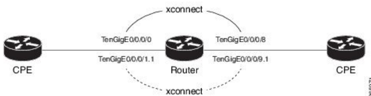
Figure 15: Local Switching Between Attachment Circuits
