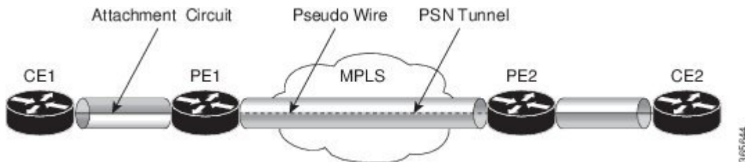
Figure 16: Static Cross-Connect Circuits in a Layer 2 VPN
