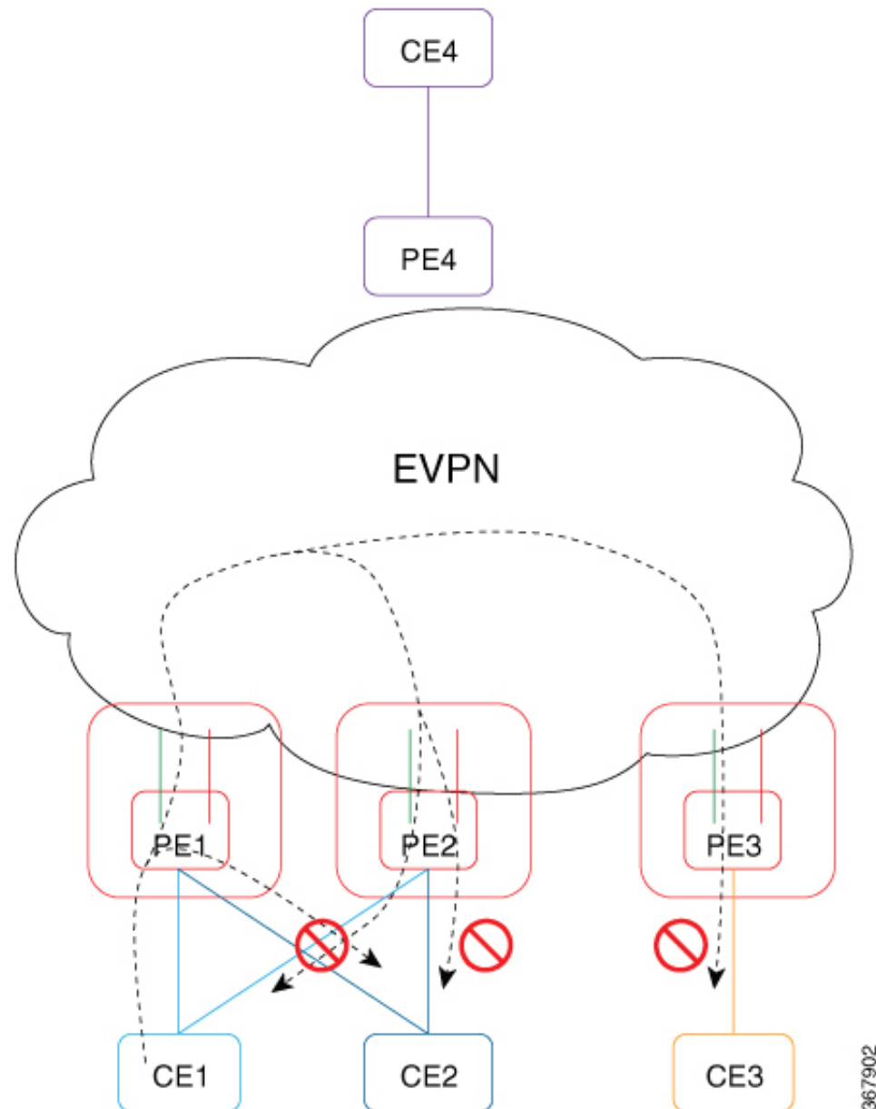
Figure 57: EVPN E-Tree
