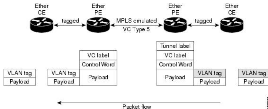
Figure 12: VLAN Mode Packet Flow
