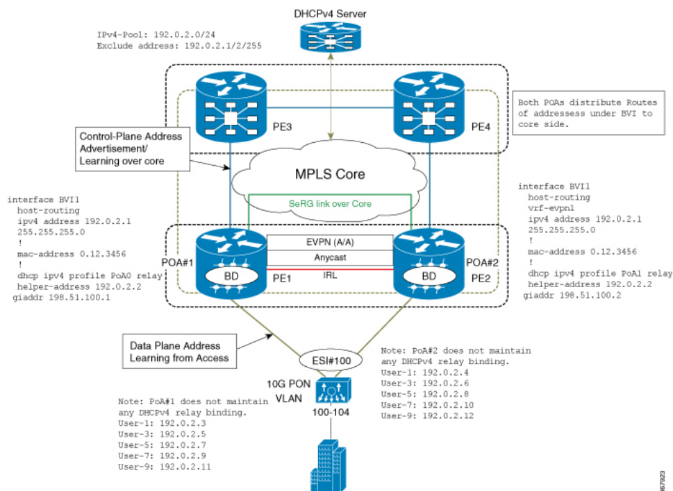
Figure 59: DHCPv4 Relay Handling for EVPN and DHCPv4 Server in Default VRF
