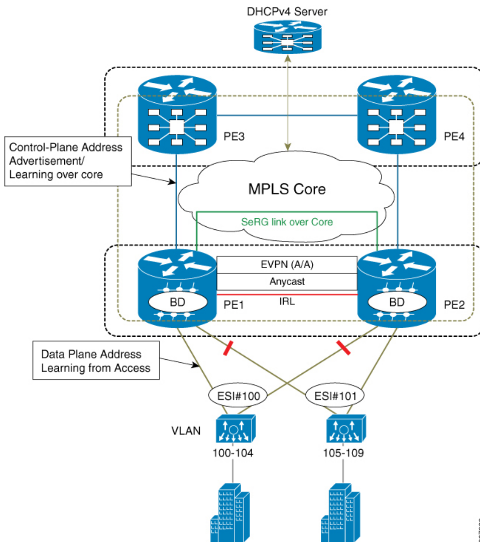
Figure 58: PON behavior in handling DHCPv4 Server for EVPN All-Active Multihoming
