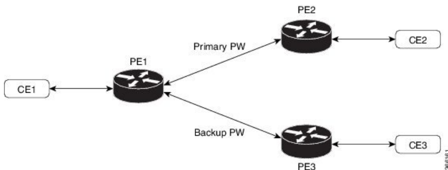
Figure 29: Pseudowire Redundancy
