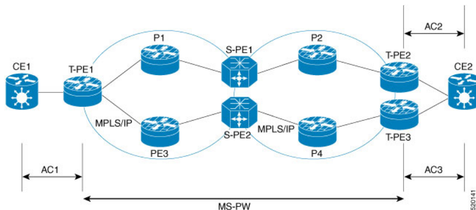
Figure 22: Multisegment Pseudowire Redundancy
