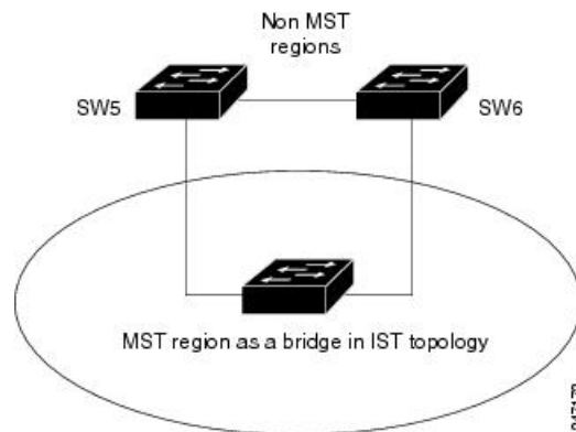
Figure 34: Logical Topology in MST Region Interacting with Non-MST Bridges
