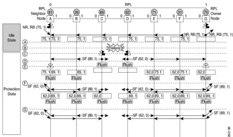
Figure 25: G.8032 Single Link Failure
