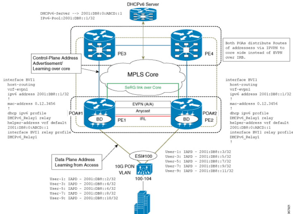
Figure 61: DHCPv6 relay Handling for EVPN and DHCPv6 Server in Default VRF
