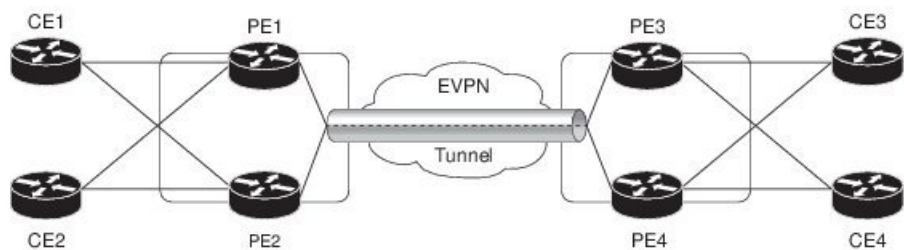
Figure 18: Flexible Cross-Connect Service Multi-Homed
