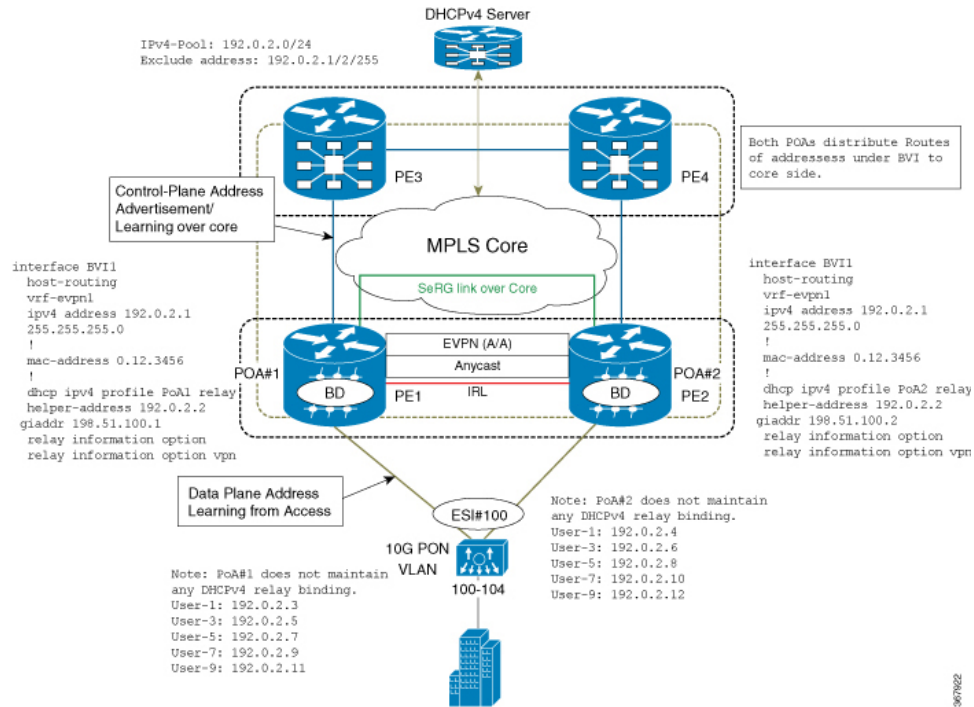
Figure 60: DHCPv4 Relay Handling for EVPN and DHCPv4 Server in Different VRF
