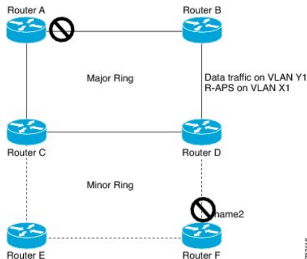
Figure 28: Open Ring Scenario
