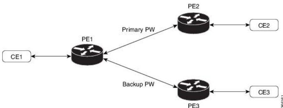
Figure 30: Pseudowire Redundancy
