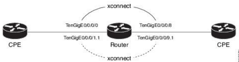
Figure 16: Local Switching Between Attachment Circuits
