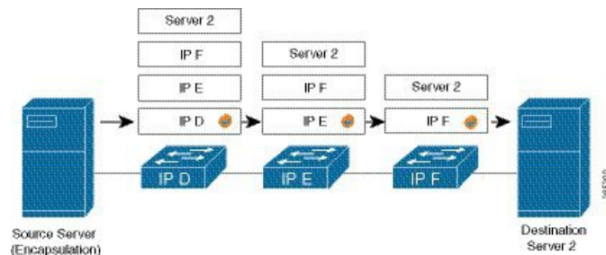
Figure 13: IP Header Decapsulation
