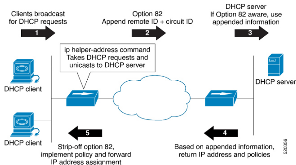
Figure 12: Forwarding Packets Using DHCP Relay Option-82
