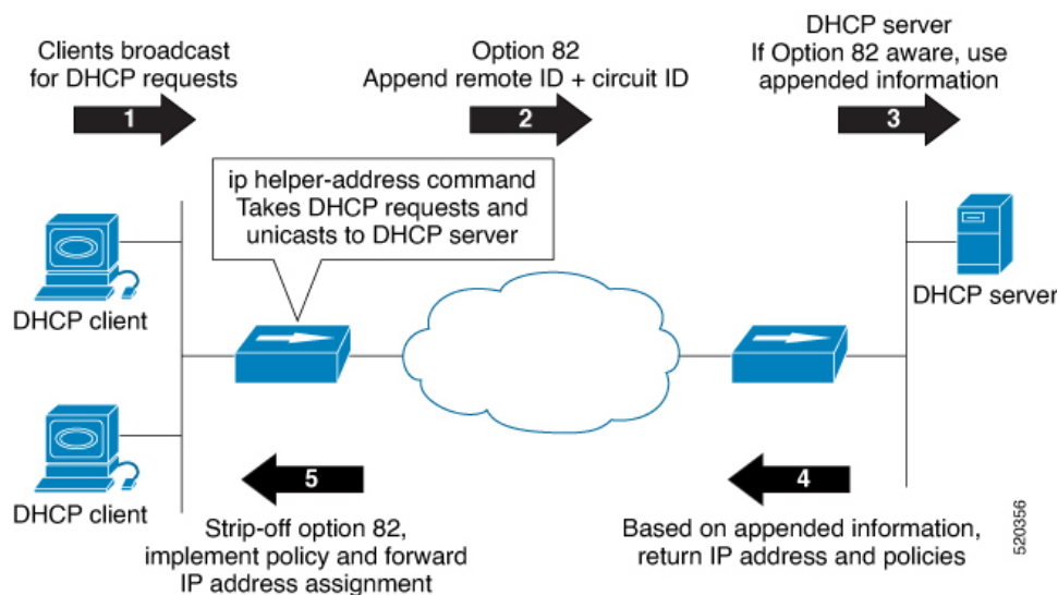
Figure 11: Forwarding Packets Using DHCP Relay Option-82
