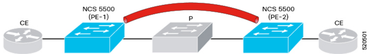
Figure 1: L2CP Tunneling
