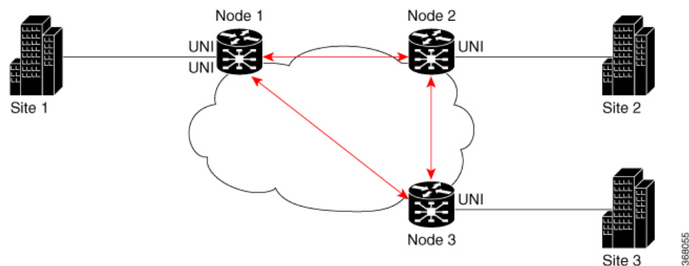
Figure 9: CFM on EVPN ELAN: Full Mesh Topology
