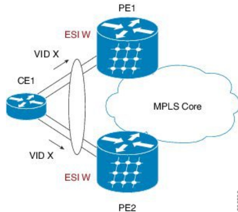
Figure 5: Dual Home Device —All-Active Load Balancing Mode
