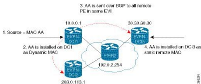
Figure 3: EVPN Software MAC Learning
