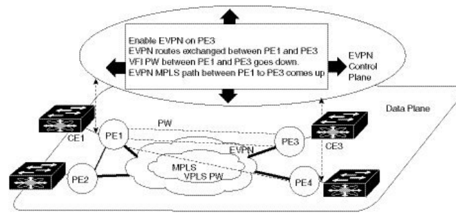
Figure 2: EVPN MPLS Seamless Integration with VPLS
