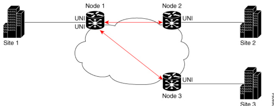
Figure 10: CFM on EVPN ELAN: Hub and Spoke Topology
