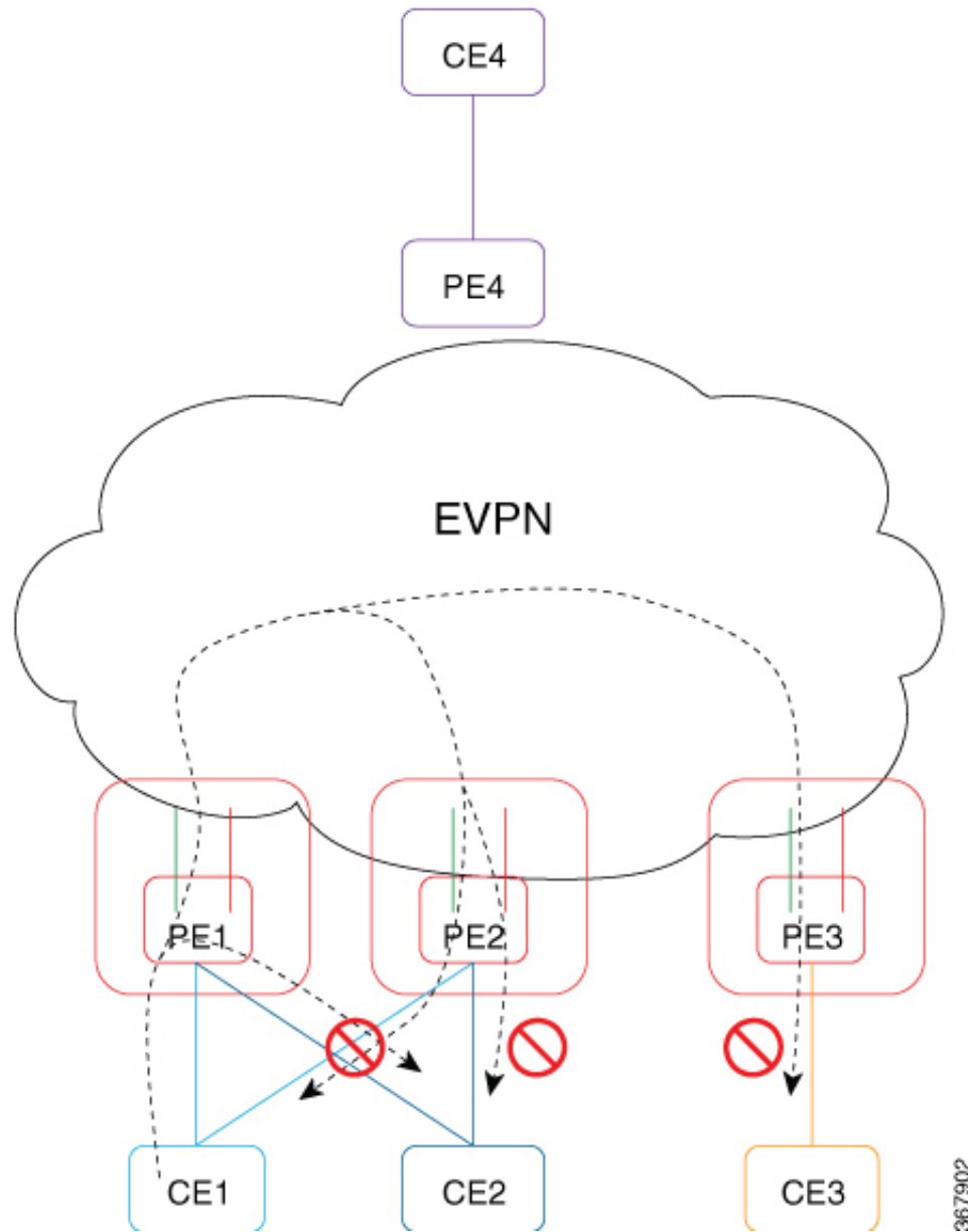
Figure 62: EVPN E-Tree
