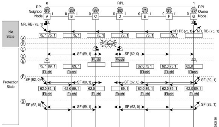
Figure 20: G.8032 Single Link Failure
