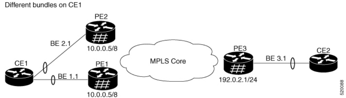
Figure 61: EVPN: Single-Active Multihoming for Anycast Gateway IRB
