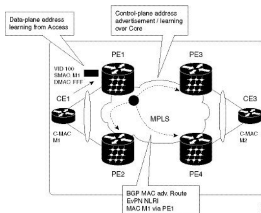
Figure 25: EVPN Operation
