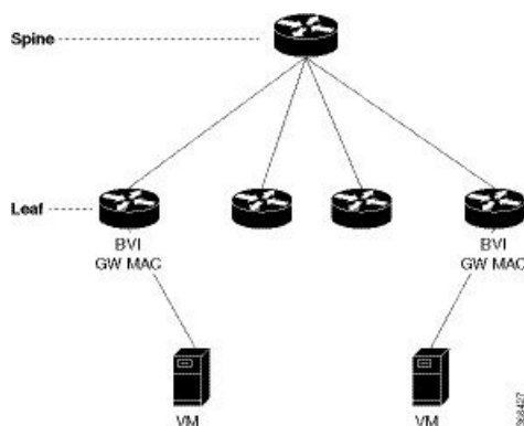
Figure 36: EVPN Single-Homing Access Gateway
