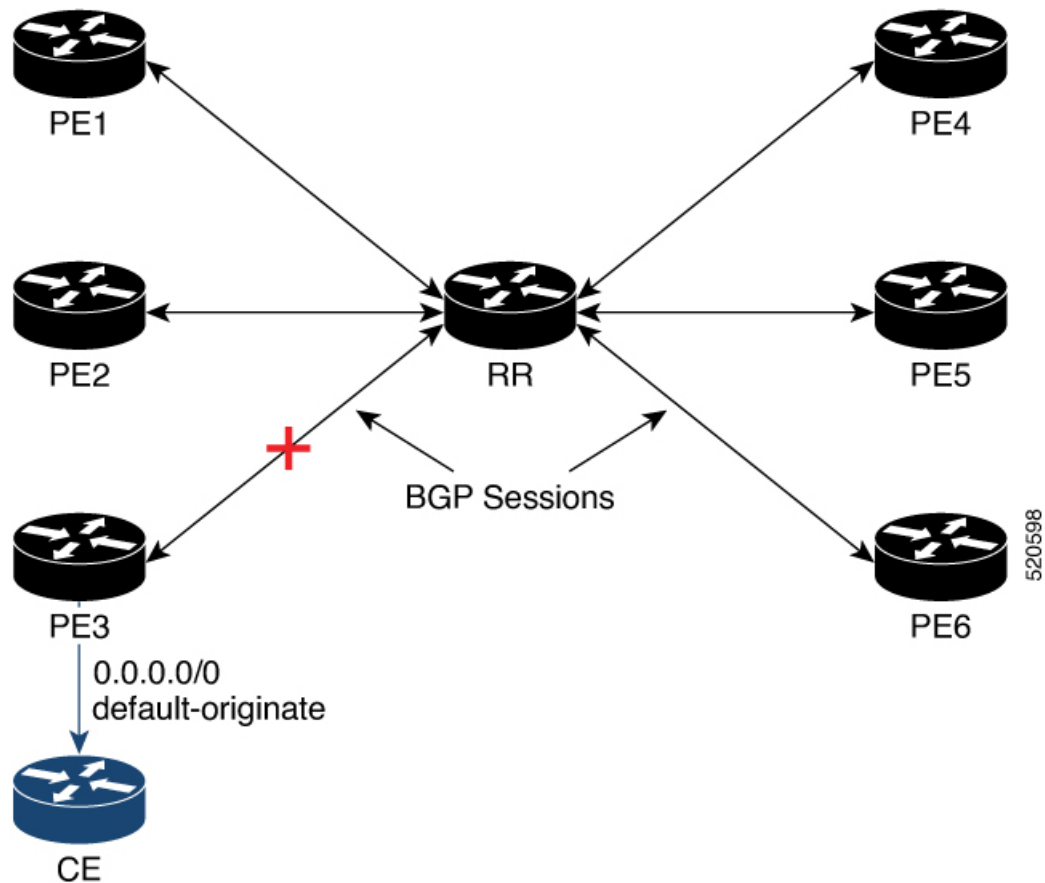
Figure 32: Advertisement of default-originate
