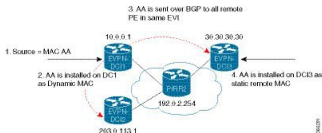
Figure 26: EVPN Software MAC Learning
