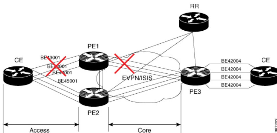
Figure 34: EVPN Core Isolation Protection
