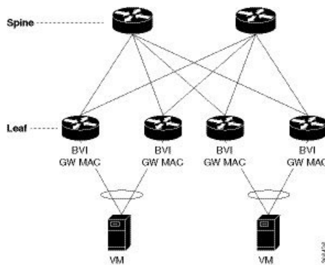
Figure 37: EVPN Multi-Homing All-Active
