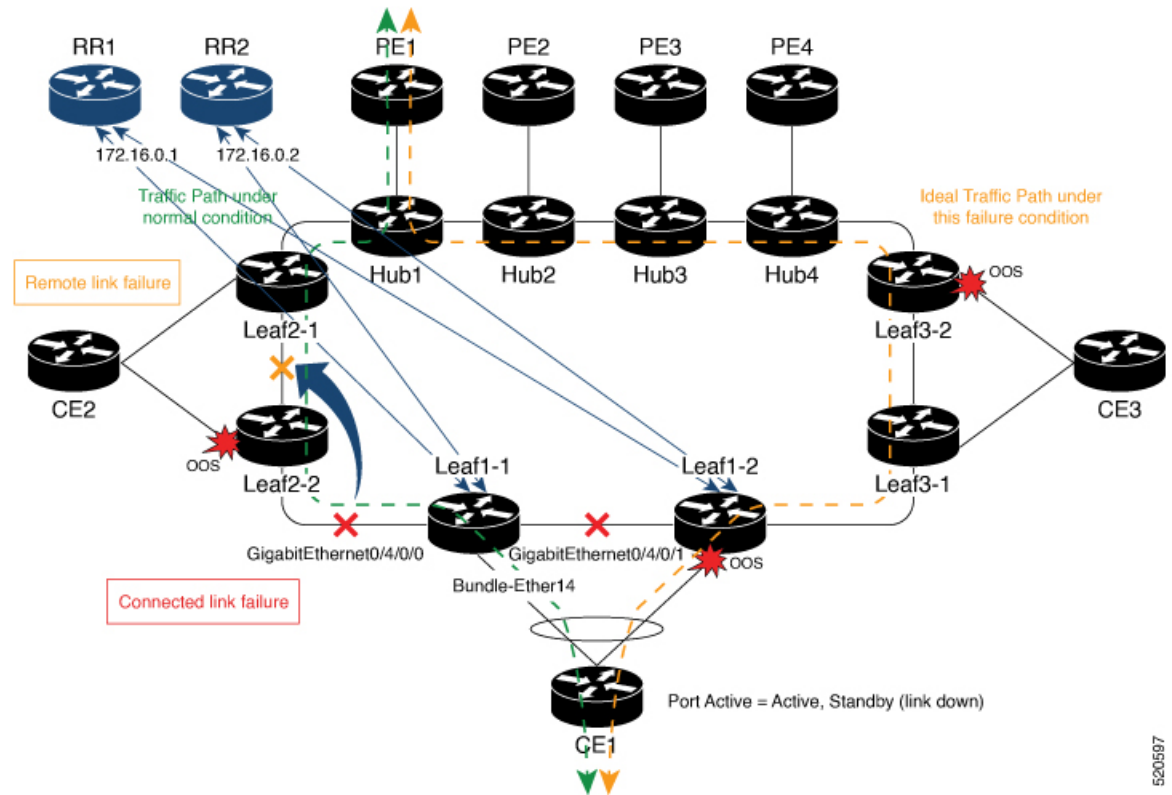
Figure 31: EVPN Convergence Using Core Isolation Protection
