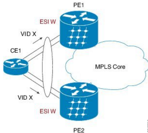
Figure 28: Dual Home Device —All-Active Load Balancing Mode
