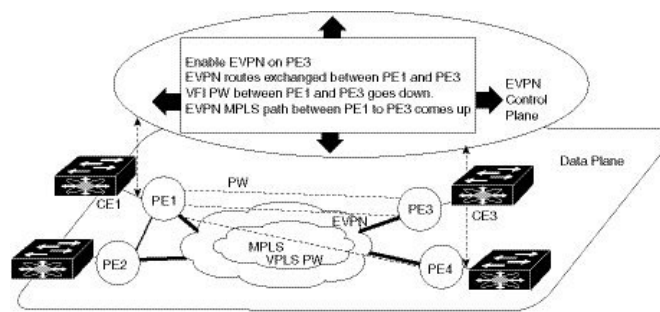
Figure 30: EVPN MPLS Seamless Integration with VPLS
