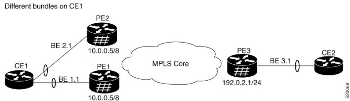
Figure 33: EVPN: Single-Active Multihoming for Anycast Gateway IRB
