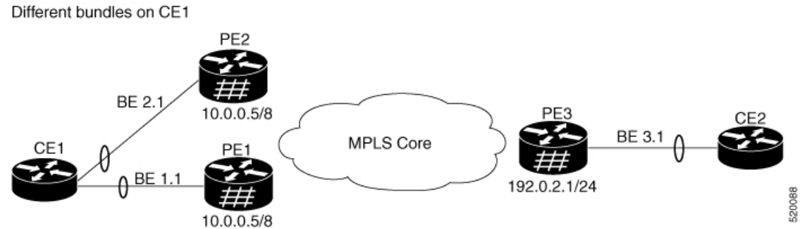
Figure 58: EVPN: Single-Active Multihoming for Anycast Gateway IRB
