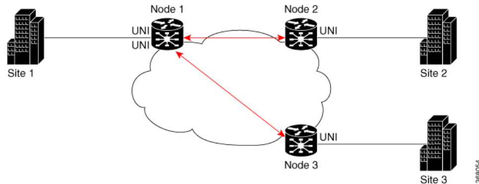
Figure 51: CFM on EVPN ELAN: Hub and Spoke Topology
