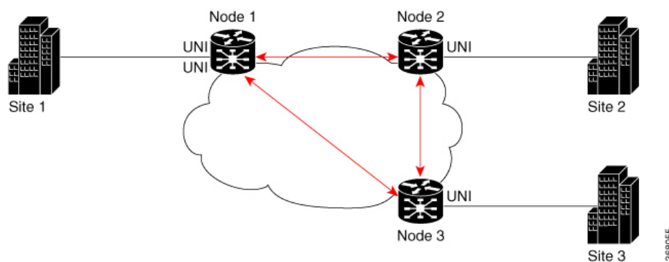
Figure 50: CFM on EVPN ELAN: Full Mesh Topology
