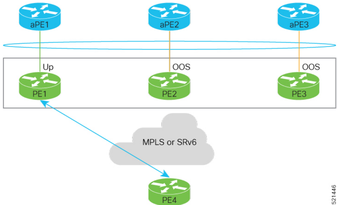
Figure 54: EVPN Access-Driven DF Election
