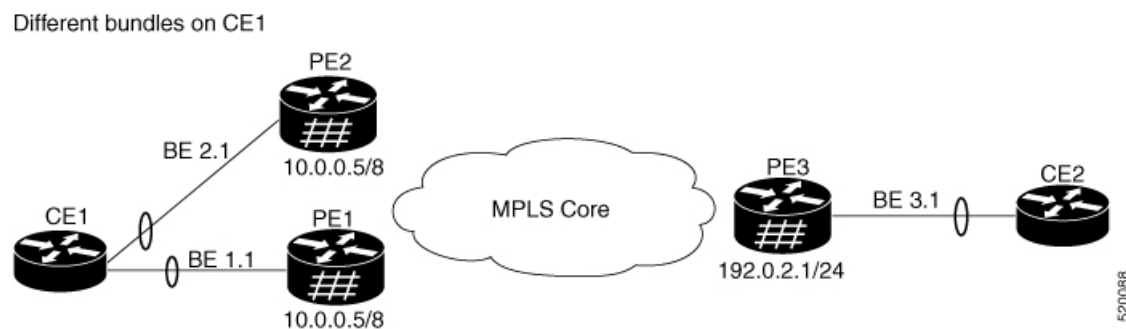
Figure 48: EVPN: Single-Active Multihoming for Anycast Gateway IRB
