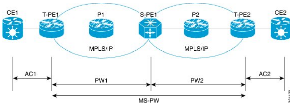
Figure 16: Multisegment Pseudowire
