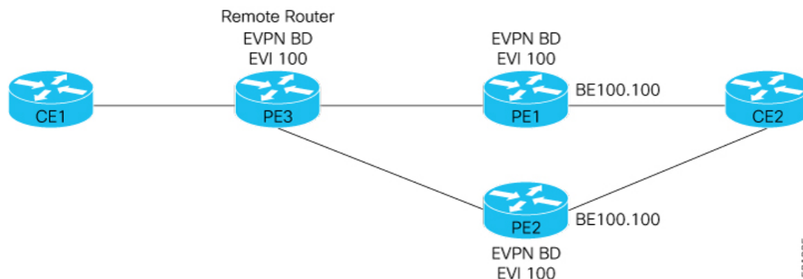
Figure 53: Layer 2 Fast Reroute
