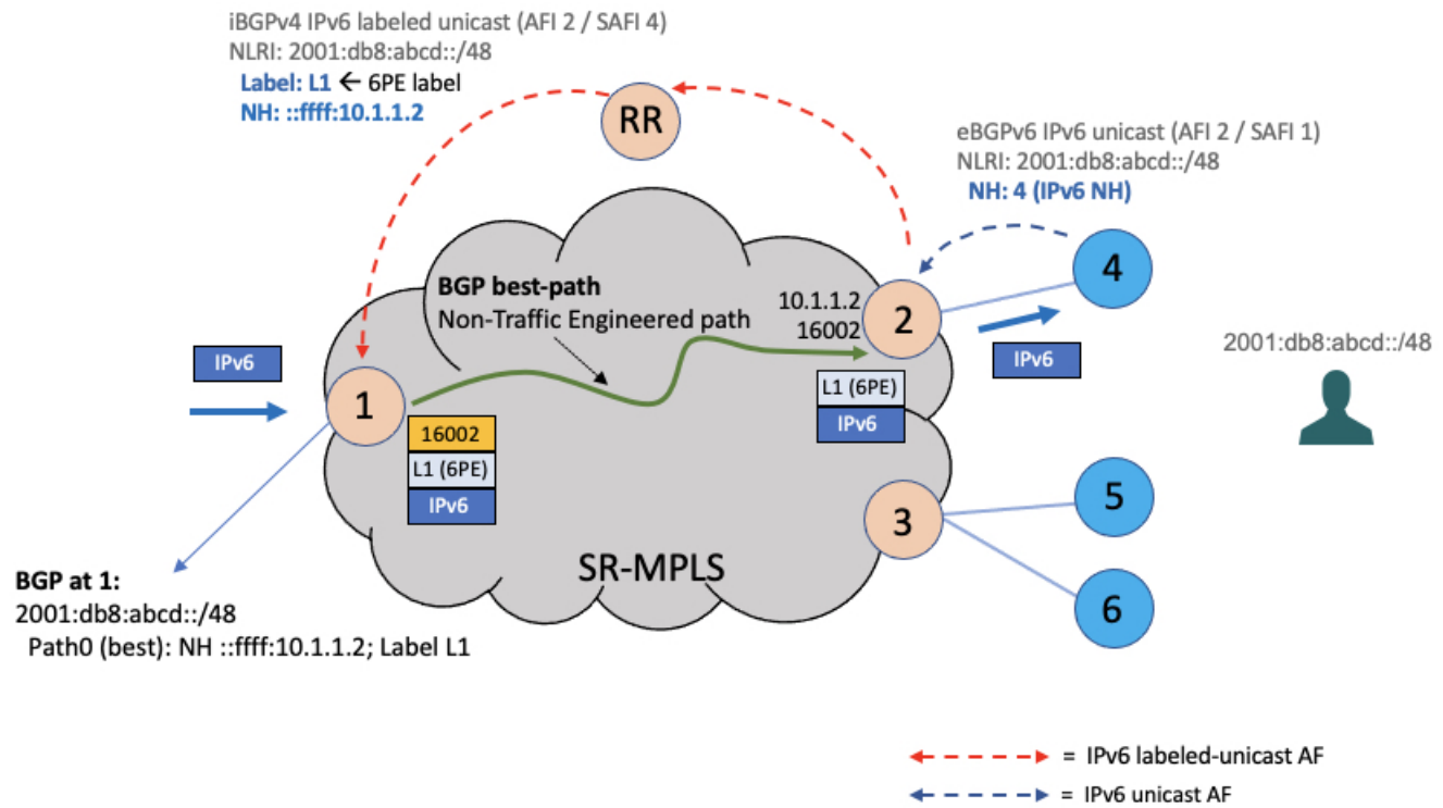
Figure 7: Steady State
