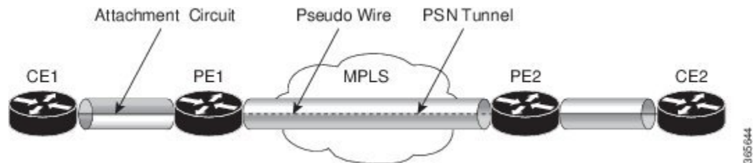
Figure 8: Static Cross-Connect Circuits in a Layer 2 VPN
