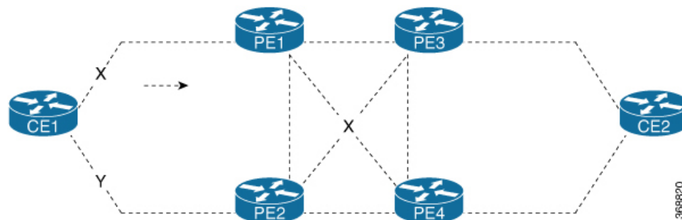
Figure 25: MAC Address Withdrawal
