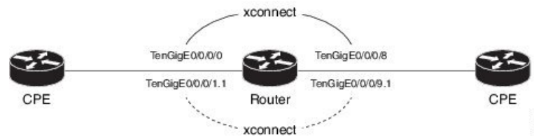
Figure 7: Local Switching Between Attachment Circuits
