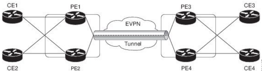
Figure 10: Flexible Cross-Connect Service Multi-Homed
