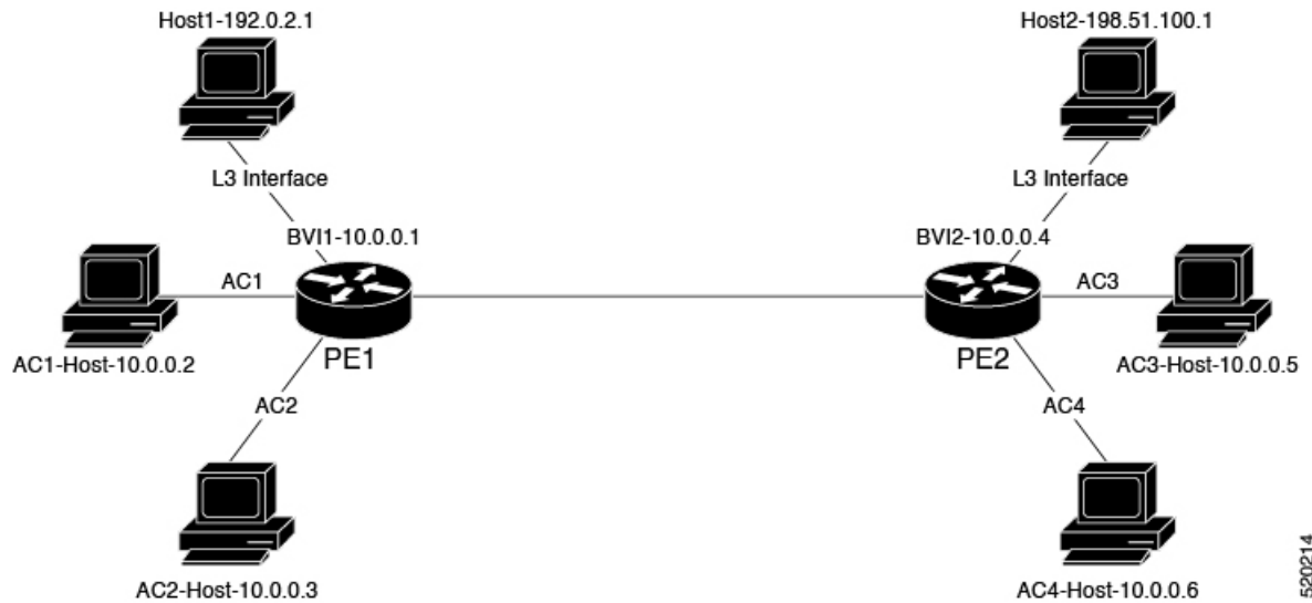
Figure 24: VPLS VFI with BVI as Routed Interface
