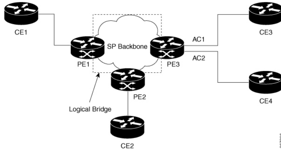
Figure 14: Split Horizon Group 2
