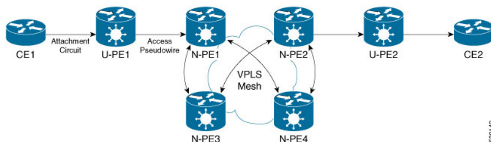
Figure 23: Access Pseudowire
