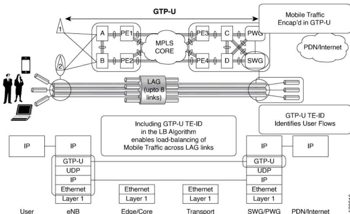
Figure 22: Mobile Transport GTP-U Load-Balancing
