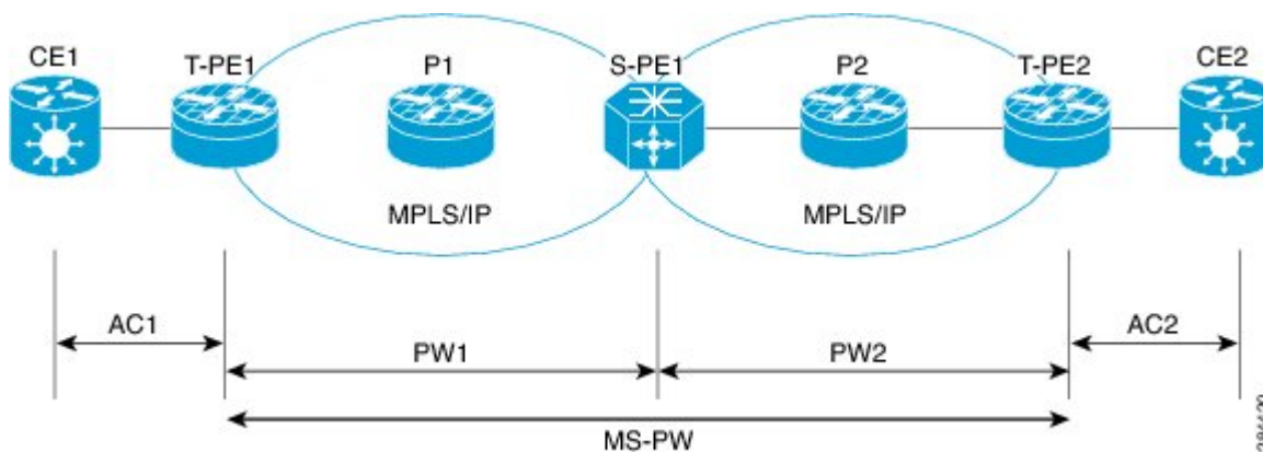
Figure 12: Multisegment Pseudowire
