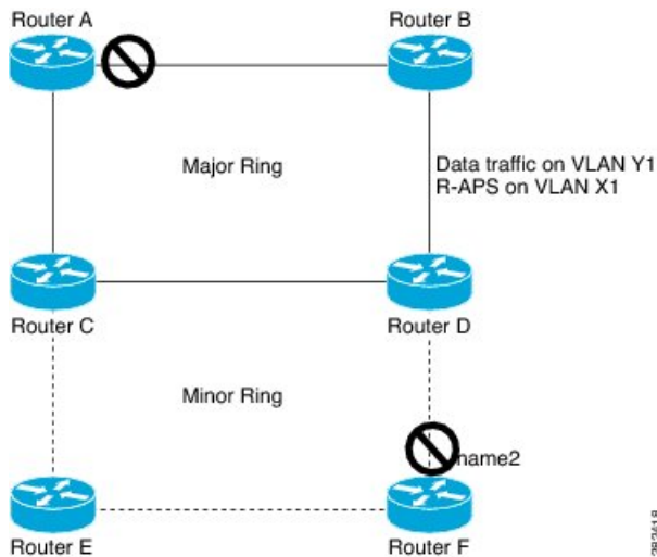
Figure 19: Open Ring Scenario
