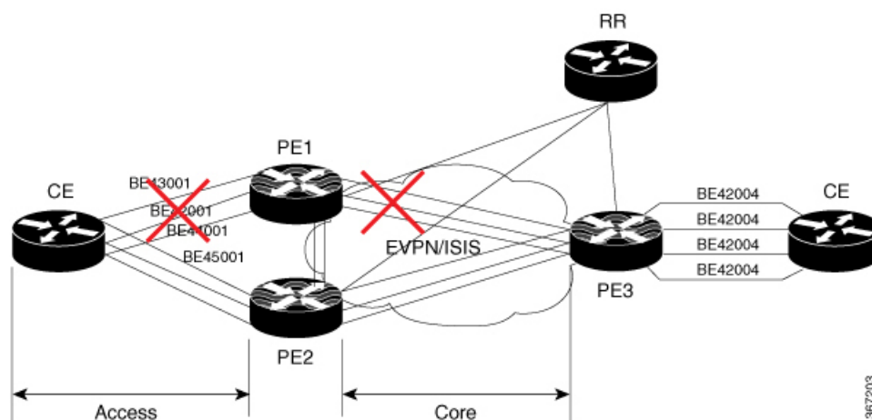
Figure 35: EVPN Core Isolation Protection
