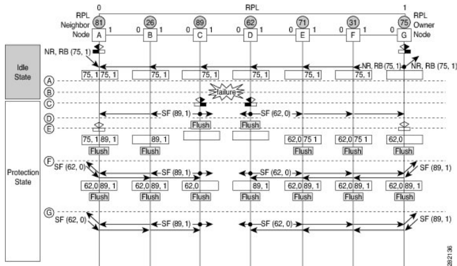
Figure 16: G.8032 Single Link Failure
