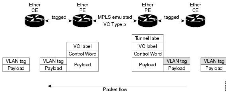
Figure 5: VLAN Mode Packet Flow
