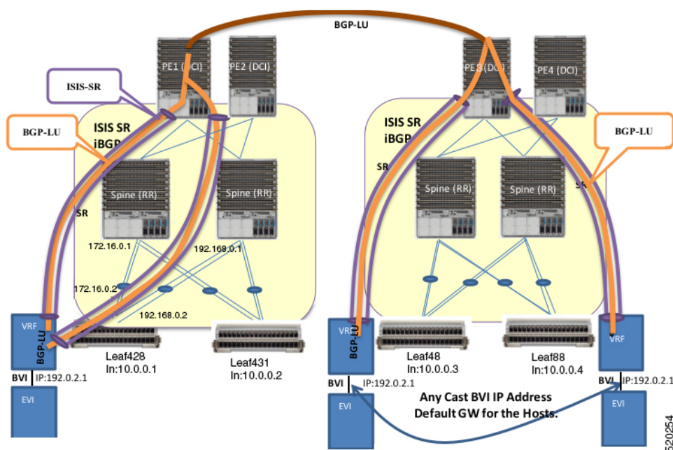
Figure 36: EVPN Bridging and VPWS Services over BGP-LU Underlay
