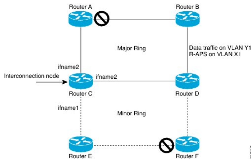
Figure 18: Open Ring Scenario - interconnection node
