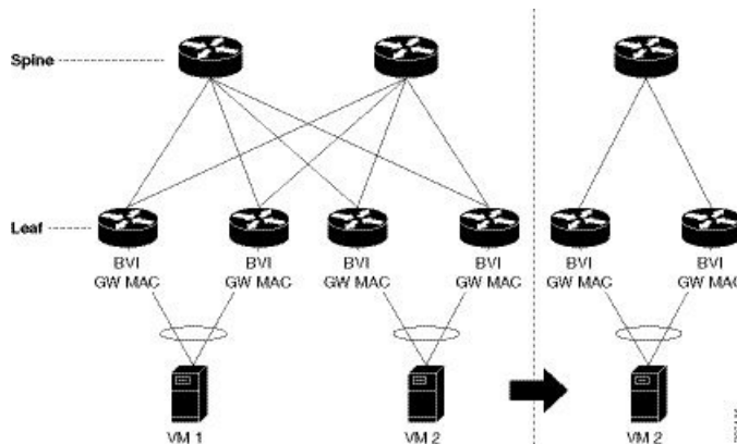
Figure 37: EVPN IRB
