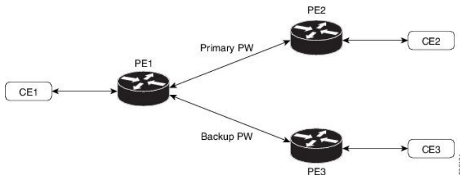
Figure 21: Access Pseudowire Redundancy
