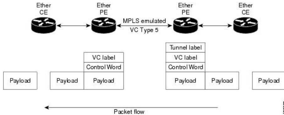
Figure 4: Ethernet Port Mode Packet Flow
