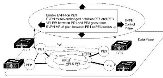
Figure 32: EVPN MPLS Seamless Integration with VPLS
