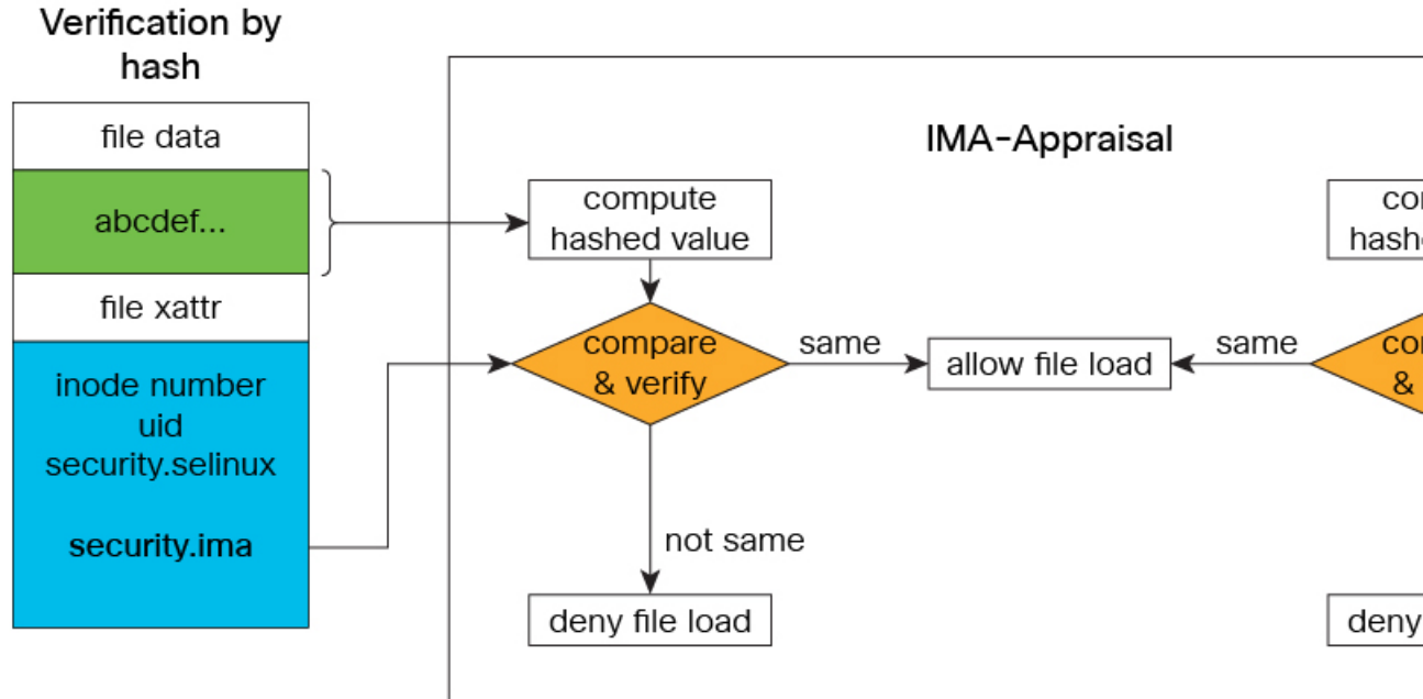
Figure 24: IMA Appraisal
