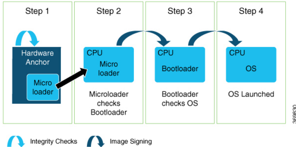
Figure 21: Secure Boot
