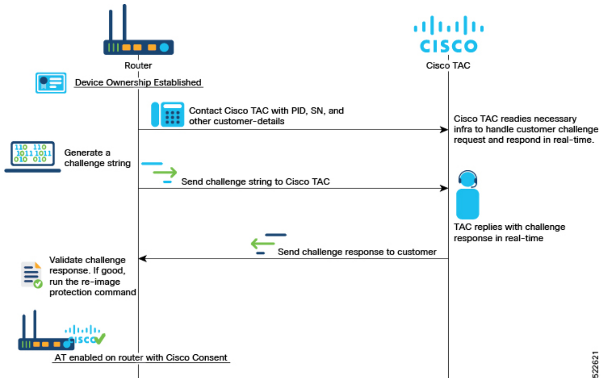
Figure 18: Workflow to Enable Reimage Protection Using Cisco Consent Token Key
