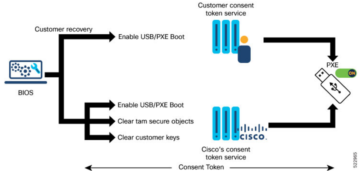
Figure 20: BIOS Recovery Utility
