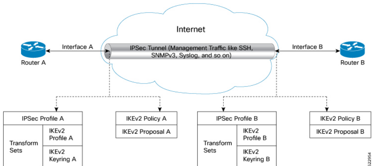
Figure 10: IPSec for Management Traffic Flow Between Two Routers
