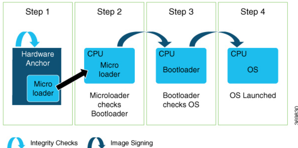
Figure 22: Secure Boot
