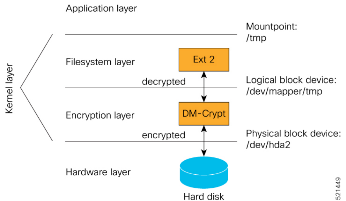
Figure 23: DM-Crypt Encryption
