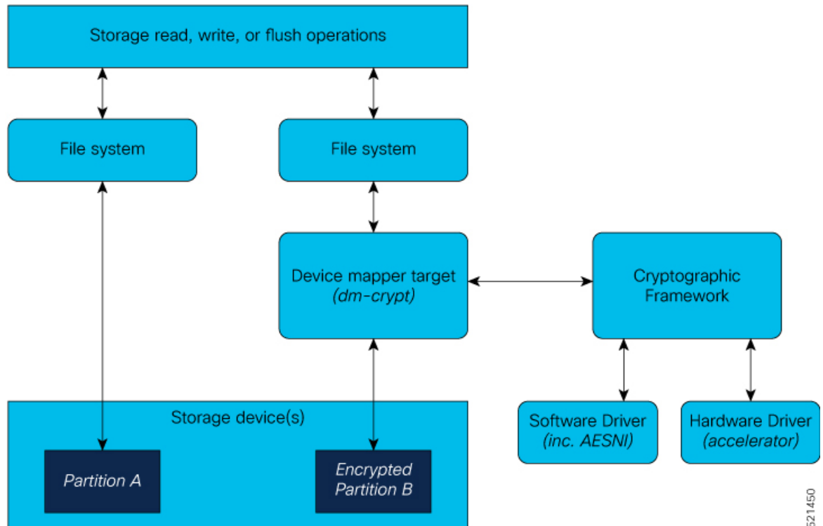
Figure 24: AES-NI Support
