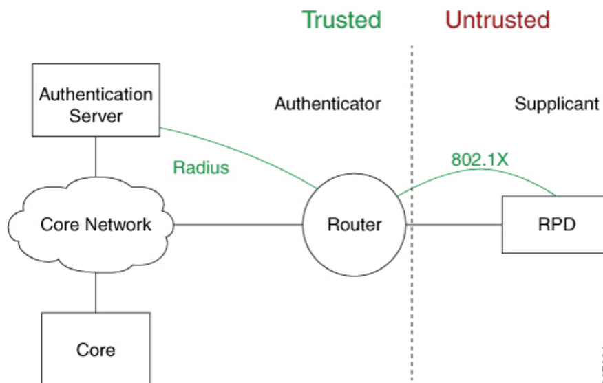
Figure 2: Topology for IEEE 802.1X Port-Based Authentication
