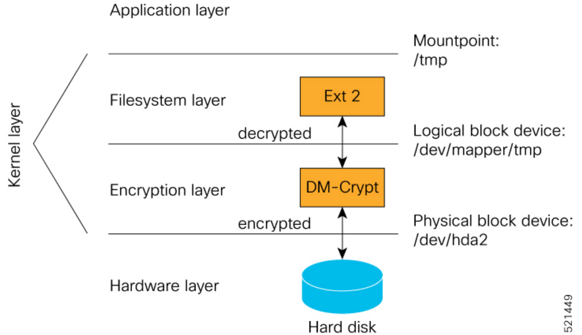
Figure 3: DM-Crypt Encryption
