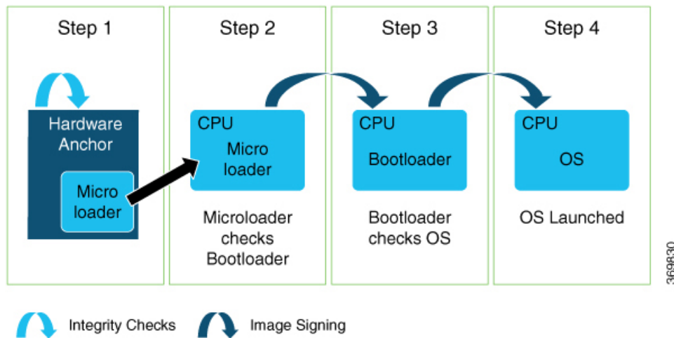
Figure 19: Secure Boot
