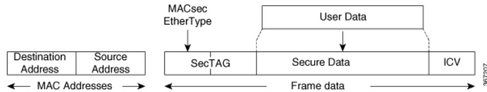
Figure 5: MACsec Frame Format
