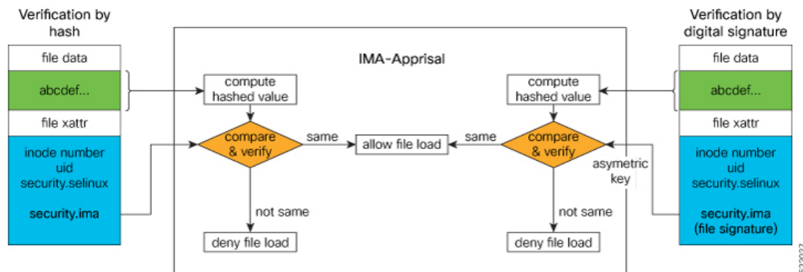
Figure 22: IMA Appraisal
