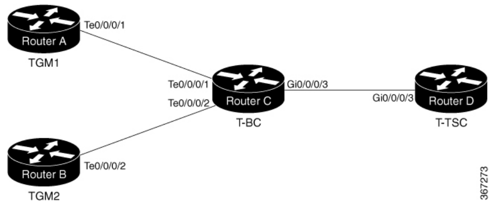
Figure 4: Sample G.8275.1 Topology
