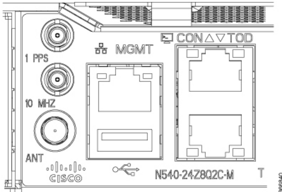
Figure 2: 1PPS, 10MHz, and the ToD ports on the Router's Front Panel
