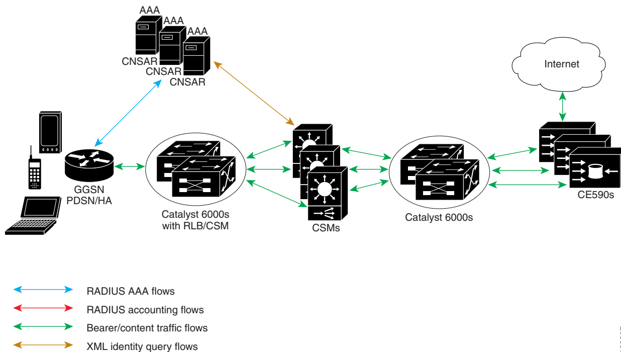
Figure 14-1 Cisco Prime AR System Overview
