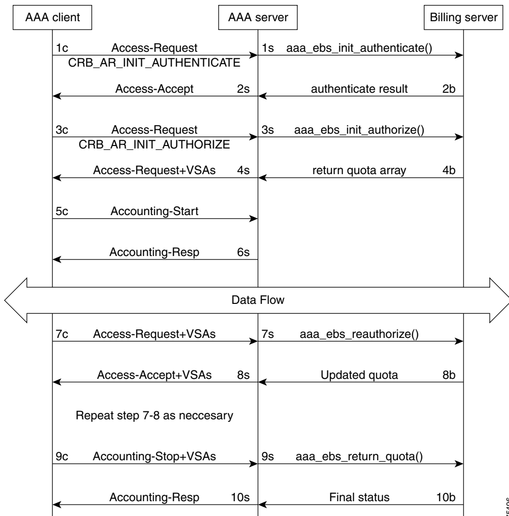
Figure 16-1 Generic Call Flow Diagram
