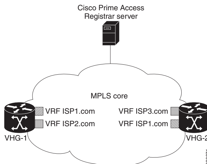
Figure 13-1 MPLS Core
