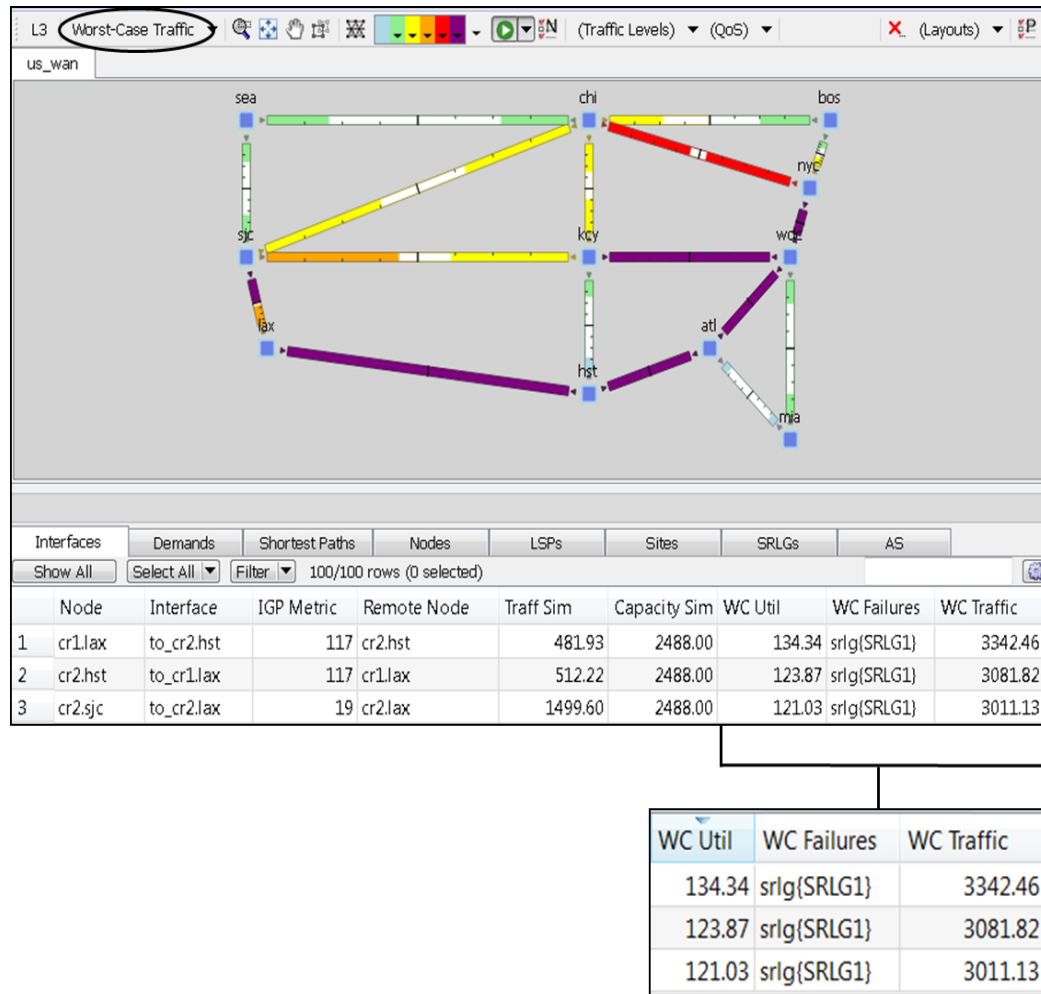
Figure 3-3 Worst-Case Simulation
